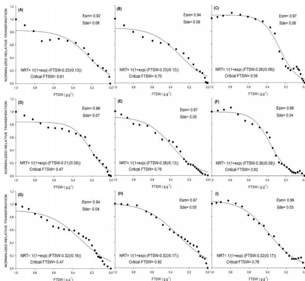
Figure 1. Normalized relative transpiration (NRT) in function of the decrease of the fraction of transpirable soil water (FTSW), in the nine clones of conilon coffee Diamante Incaper ES8112 ("A"- Clone 101; "B"- Clone 102; "C"- Clone 103; "D"- Clone 104; "E"- Clone 105; "F"- Clone 106; "G"- Clone 107; "H"- Clone 108; "I"- Clone 109).
