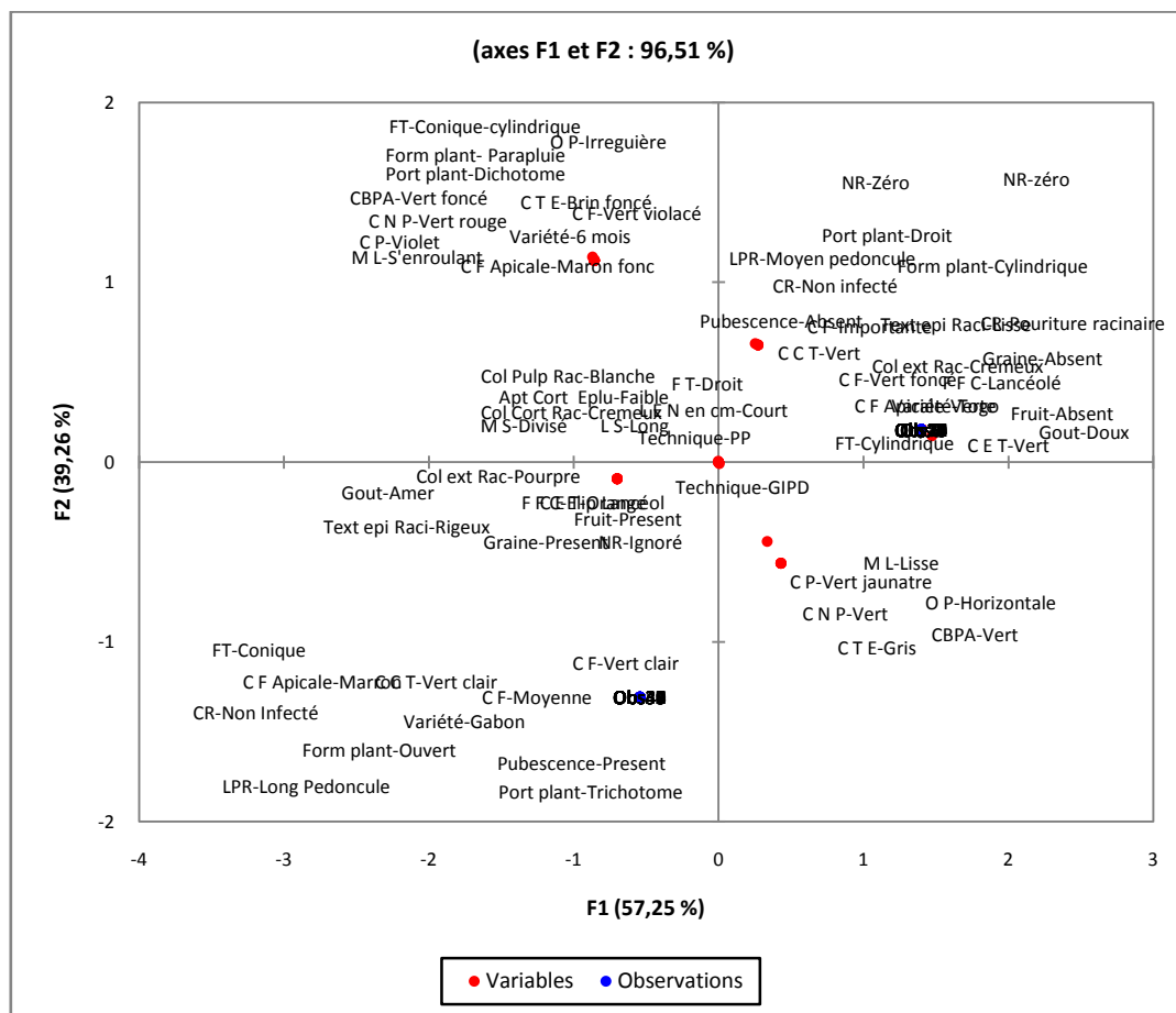
Figure 5: Multiple analysis of correspondence of agro-morphological descriptors
