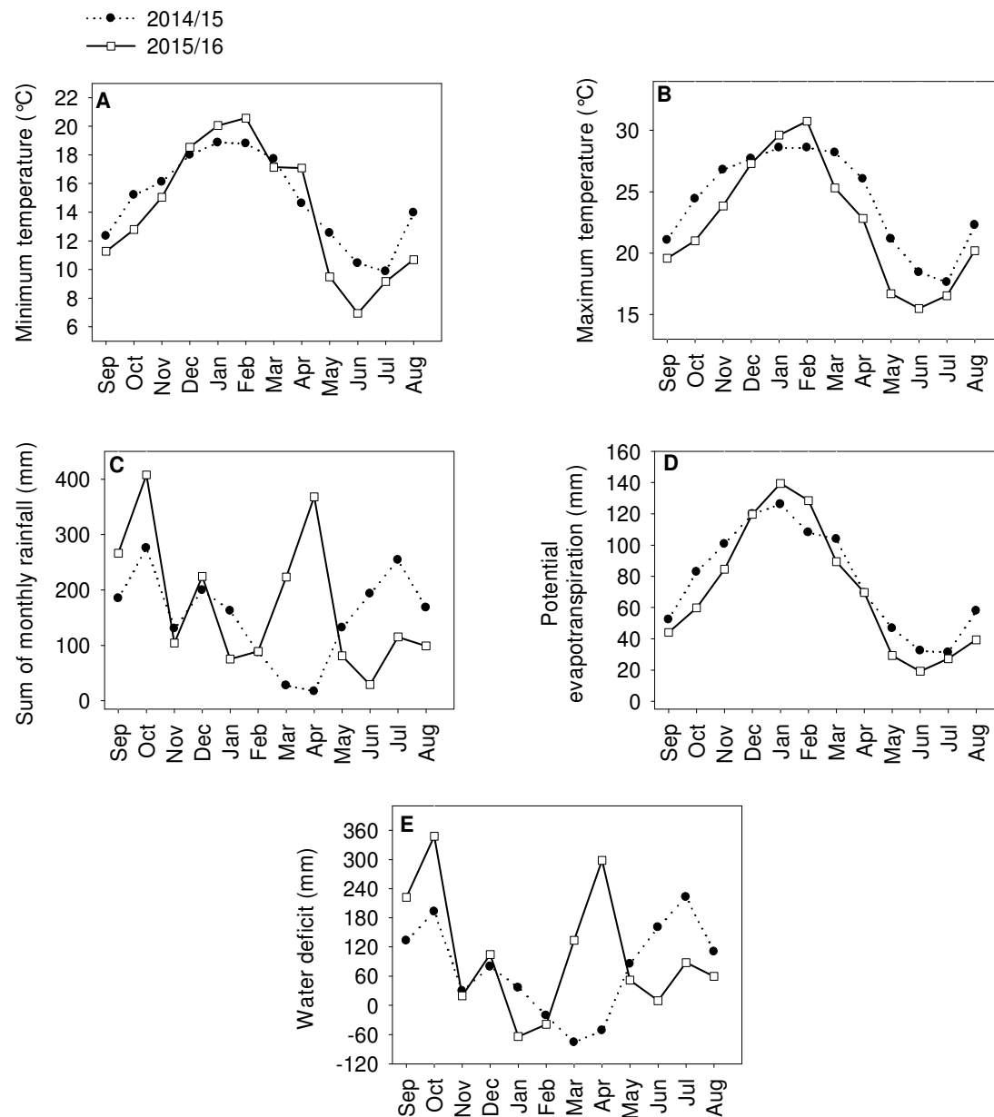
Figure 1. Monthly average of minimum (A) and maximum (B) temperatures, monthly averages, sum of monthly rainfall (mm) (C), potential evapotranspiration (mm) (D) and water deficit (mm) (E) between the months of September and August of 2014/15 and 2015/16, obtained from Meteorological Station of Bagé, RS.
