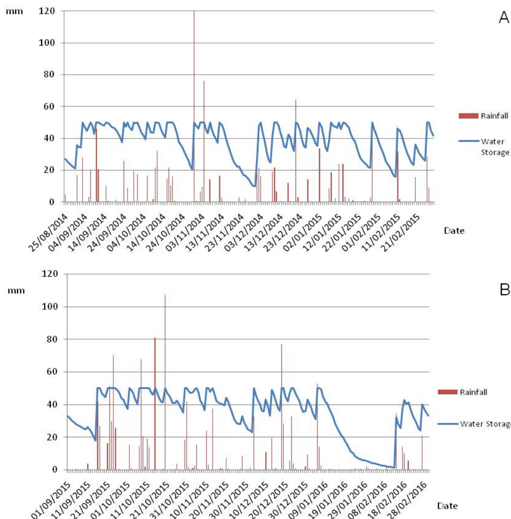
Figure 2. Water storage in the soil and rainfall (mm), obtained between September and March 2014/15 (A) and 2015/16 (B), from Meteorological Station of Bagé, RS.
