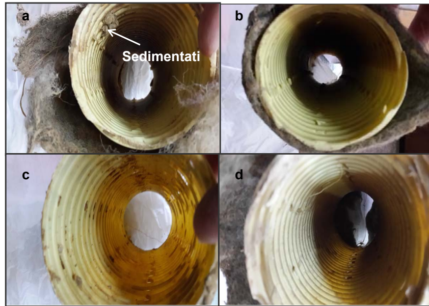
Fig. 8. Example of the excavation results of the tested drain lines
