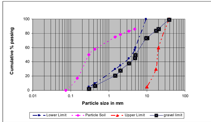
Fig. 7. Representative curve of granular drain envelope material
