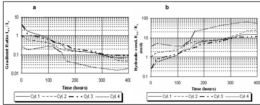
Fig. 4. Permeameter test results for El-Bostan area
