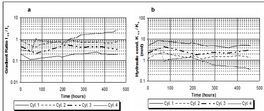
Fig. 3. Permeameter test results for Fabes area
