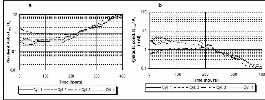
Fig. 5. Permeameter test results for Abu-Masoud area
