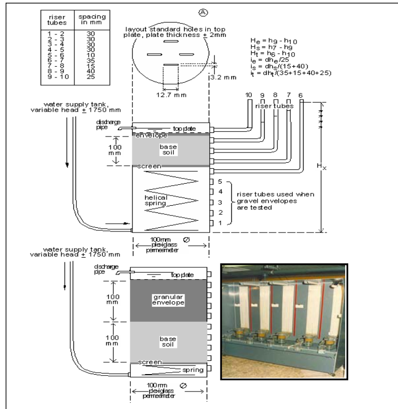
Fig. 2. Upward flow permeameter [11]
