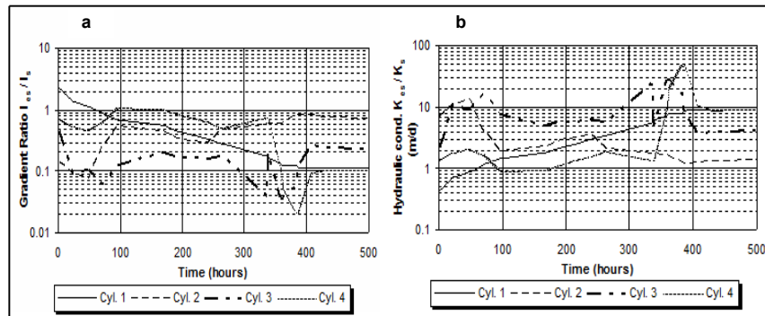
Fig. 6. Permeameter test results for El-Ameria area
