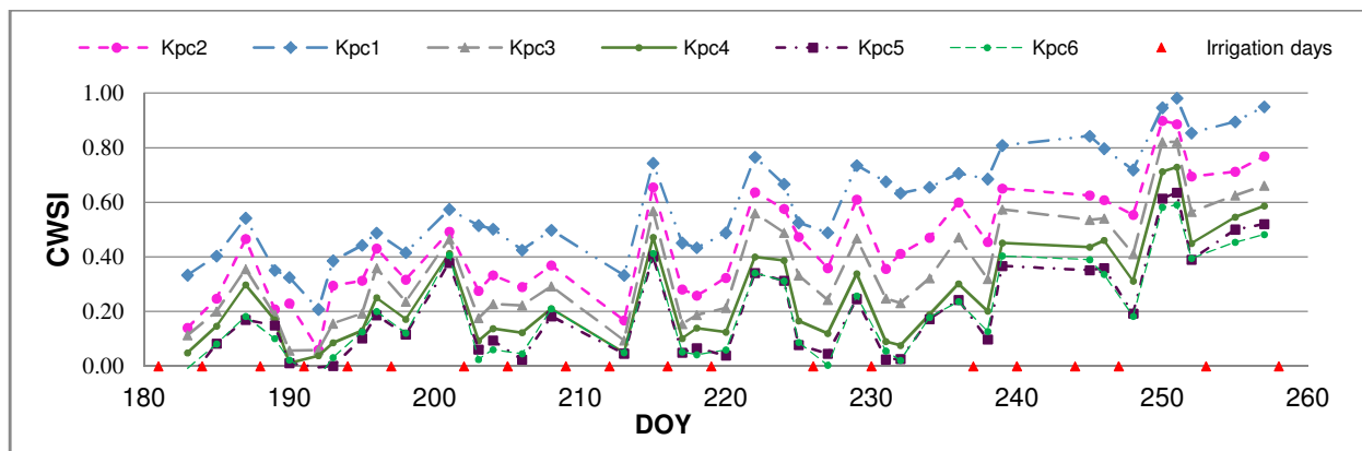
Figure2. The crop water stress index (CWSI) for each irrigation treatment
