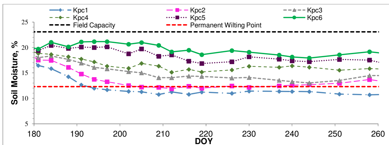
Figure3. Soil moisture content before irrigation
