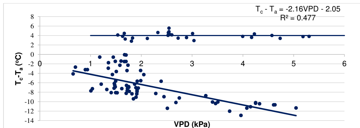
Figure 1. Upper and lower baselines for soybean
