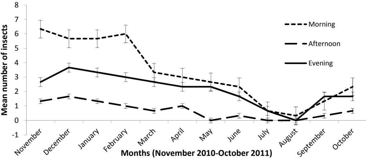
Fig 4: Monthly mean numbers ( \pm SEM) of major Hemiptera insect pests in cocoa farms at 07:00-09:00 (morning), 12:00-13:00 (afternoon) and 17:00-18:00 (evening) at (A) Ekona and (B) Muyuka for November 2010-October 2011
