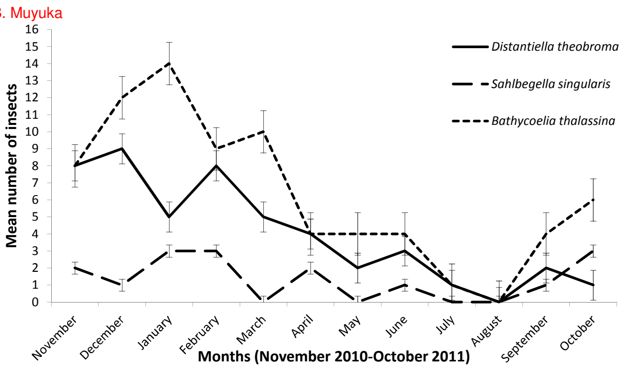
161 Fig 3. Monthly mean numbers ( \pm SEM) of major Hemiptera insect pests in cocoa farms at (A) Ekona and 162 163 (B) Muyuka for November 2010-October 2011
