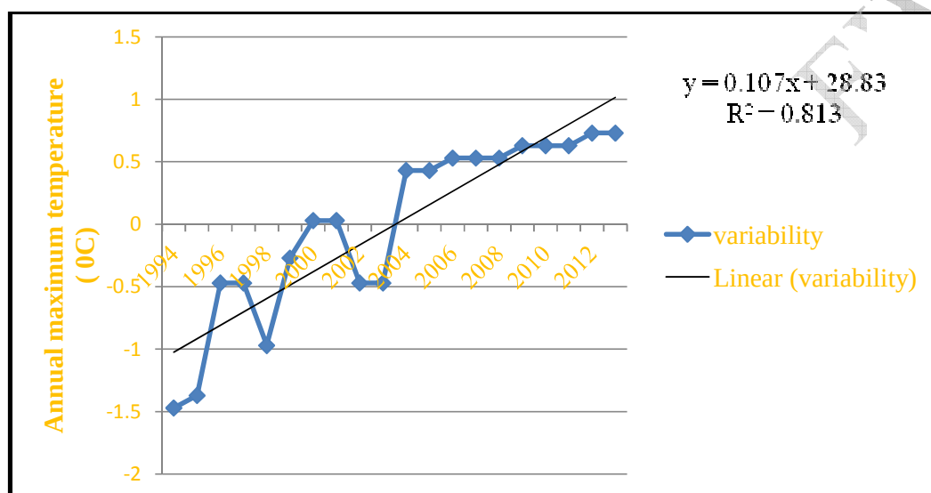
Figure 2: Inter-annual maximum temperature anomaly (1994-2013)
