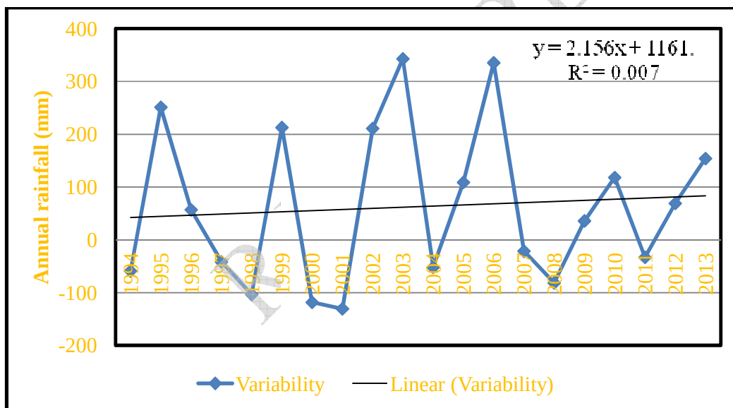
Figure 3: Inter-annual rainfall anomaly (1994-2013)
