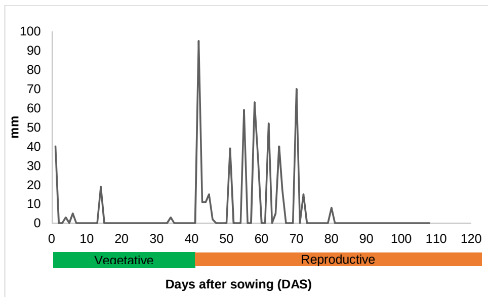
55 Fig. 1. Rainfall, in millimeters, from November 2015 to April 2016 [Nazimah3] .
