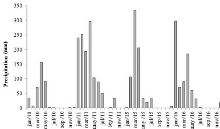
Fig. 2. Precipitation occurred at the meteorological station of the municipality of Marco in the years 2010, 2011, 2015 and 2016 [12]
