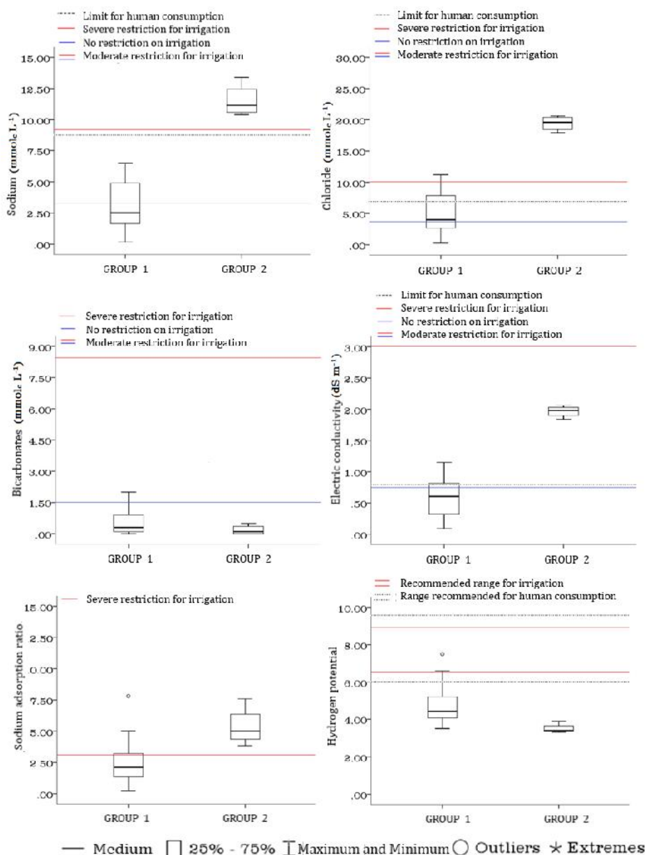
Fig. 5. Statistical analysis of descriptive attributes studied for groundwater supplies at the perimeter irrigated low Acaraú – CE
