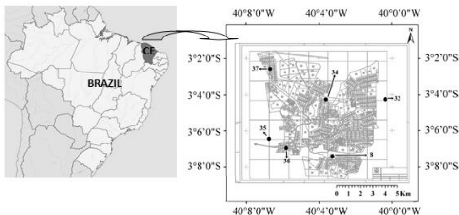
Fig. 1. Localization of irrigated perimeter of lower Acaraú-CE.
