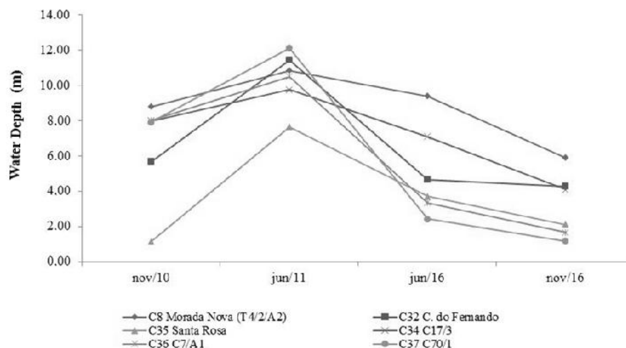
Fig. 3. Variation of groundwater in perimeter irrigated Low Acaraú-CE.
