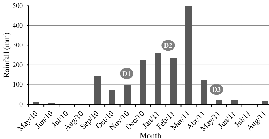
Figure 1. Monthly rainfall accumulation in the catchment of Córrego Rico (SP) where water samples were collected for herbicide detection. Sampling dates: D1: November 26 to 30, 2010, D2: February 02 to 06, 2011, D3: May 15 to 18, 2011. Jaboticabal, SP.
