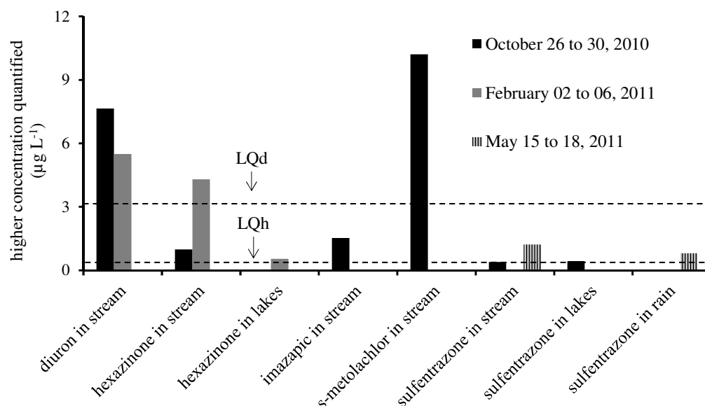
Figure 2. Residual maximum of herbicides, quantified by LC-MS / MS in water samples collected on three occasions under three matrices (rain, streams and lakes), in the watershed of Córrego Rico, Jaboticabal, SP, Brazil. Limit of quantification for diuron (LQd) and other herbicides (LQh).
