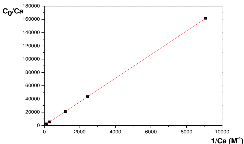
Figure 9. C_0/Ca versus 1/Ca
