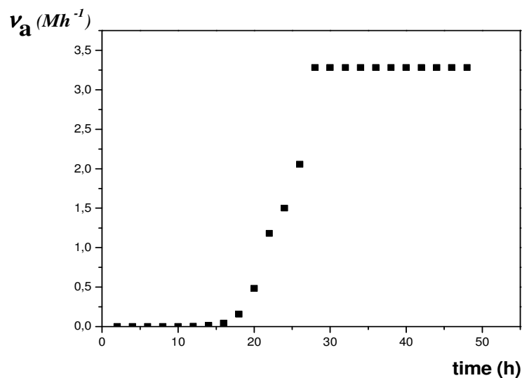
Figure 4a. v_a versus time
