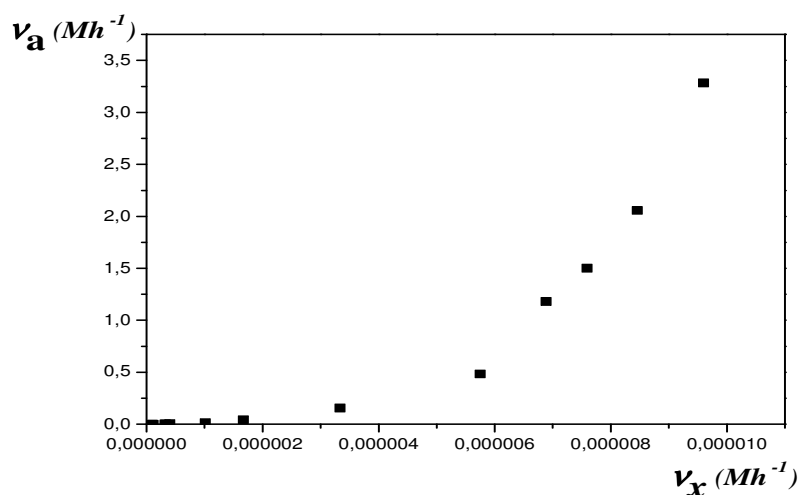
Figure 2b. v_a versus v_x
