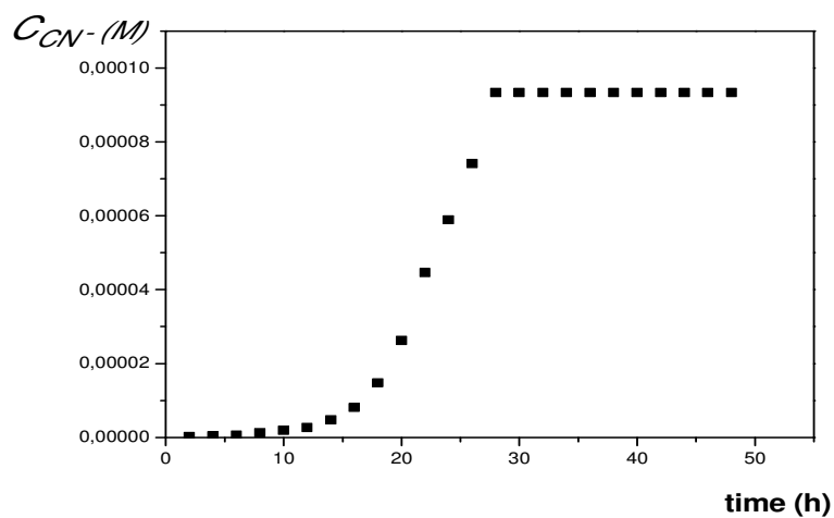
320 Figure 8. C_{CN^-} versus time
