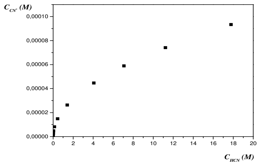
Figure 3. C_{CN^-} versus C_{HCN}
