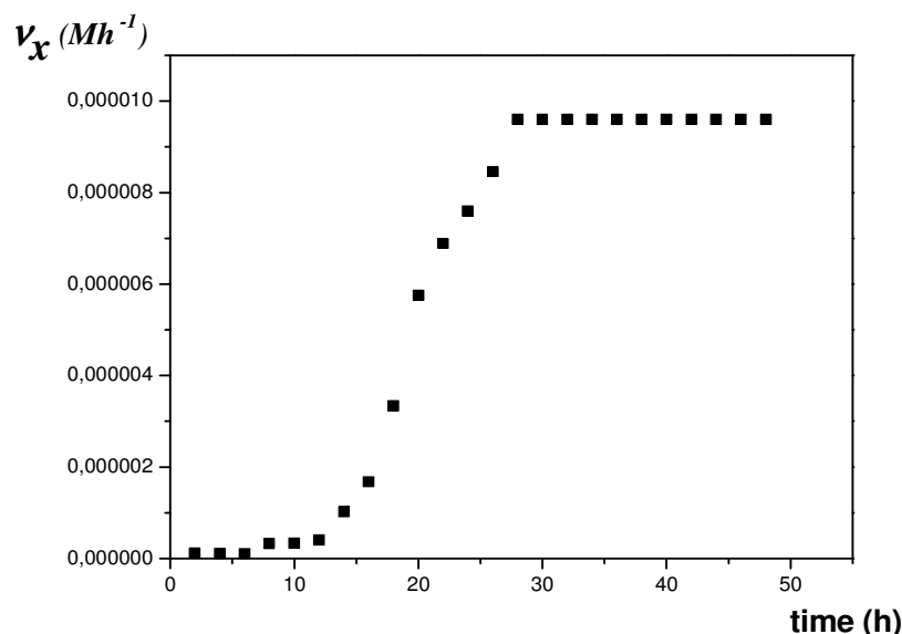
Figure 4b. v_x versus time
