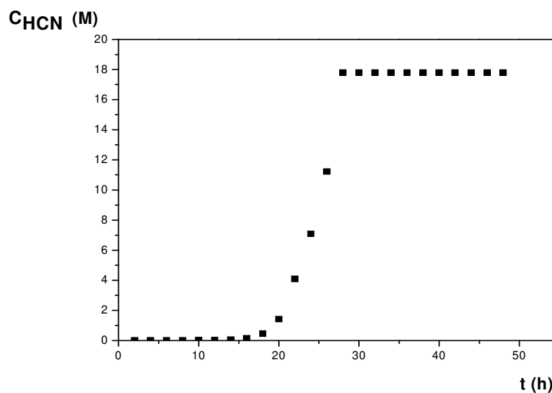
Figure 7. C_{HCN} versus time
