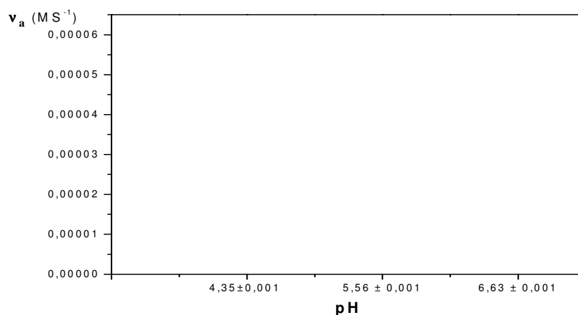
Figure 6. V_a versus pH
