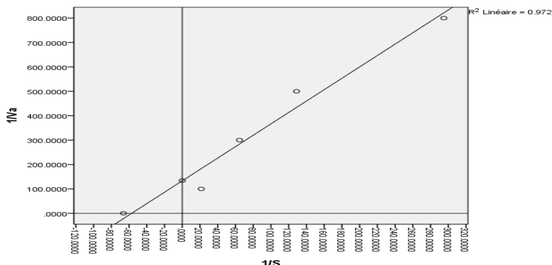
Figure 5. \frac{1}{V_a} versus \frac{1}{[S]}
