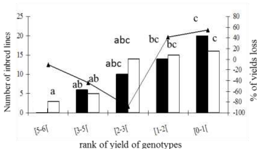
Fig. 2. Yield and yield loss of the best inbred lines on acidic and corrected soil at Nkolbisson.
