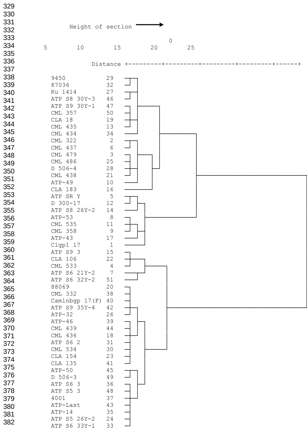
Fig.5. Dendrogram obtained by linkage between groups and by the non-hierarchical classification process of endogamous genotypes at Nkoemvone.
