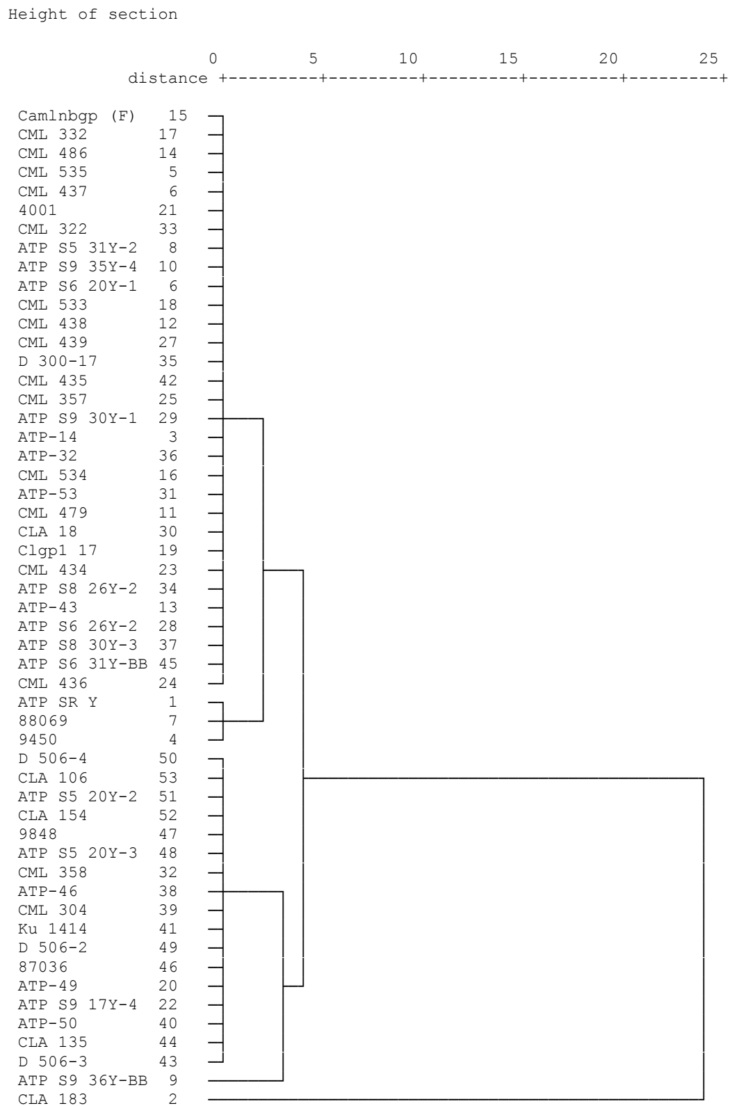
Fig.4. Dendrogram obtained by linkage between groups and by the non-hierarchical classification process of endogamous genotypes at Nkolbisson.
