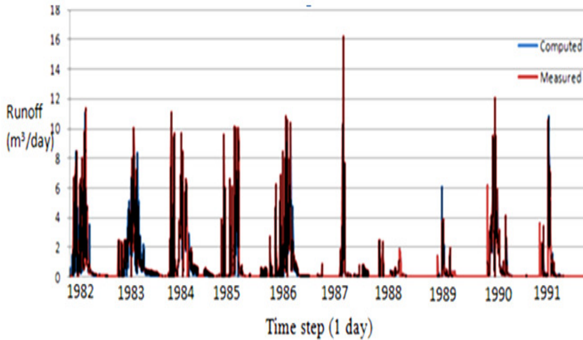
Figure 6: Hydrographs of simulation using adjusted catchment parameters and time constants
