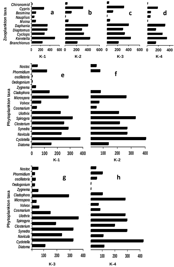
180 181 182 Figure 3. Zooplankton (a, b, c, d) and phytoplankton (e, f, g, h) community and their 183 abundance in ponds K 1 , K 2 , K 3 and K 4 . 184
