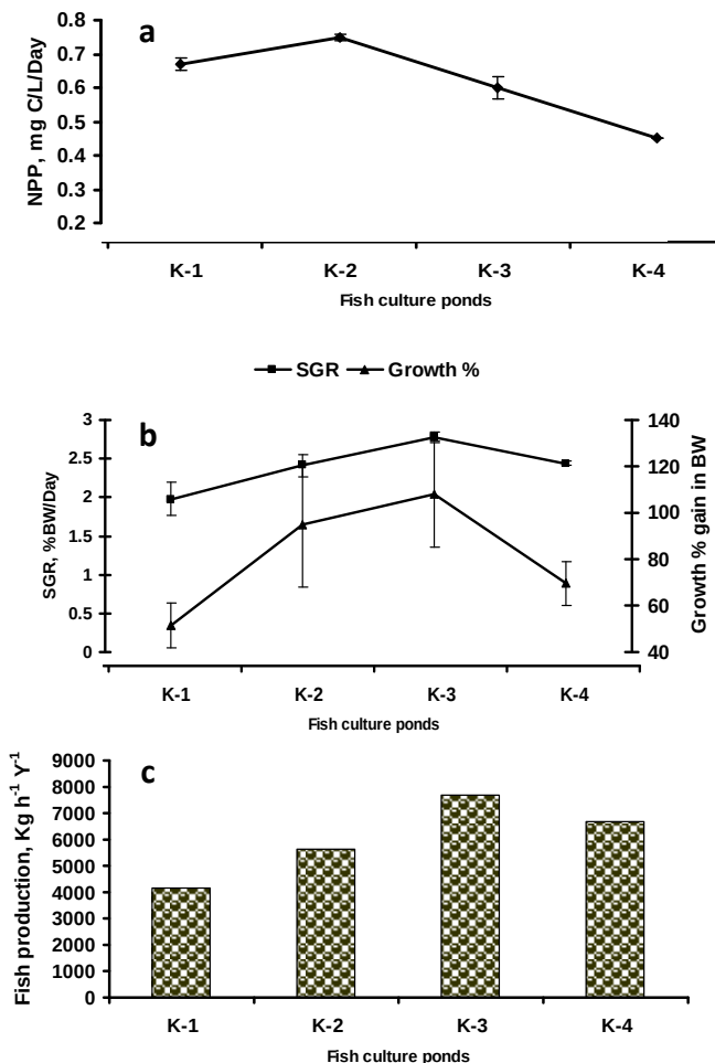
Figure 2. Plots showing the net primary productivity (NPP) (mg C/L/Day), fish growth (Specific Growth Rate (SGR)), growth percentage gain in body weight (%BW/Day) and fish production (Kg/hectare/year) for the two unmanaged ponds (K 1 and K 2 ) and two managed ponds (K 3 and K 4 ) in the district of Kurukshetra, Haryana, India.
