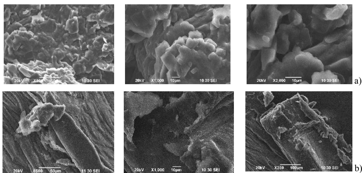
Fig.10. Scanning Electron Microscopy (SEM) of Formulations a) LEIM-3 and b) LTFH-4 at Different Magnification Respectively
