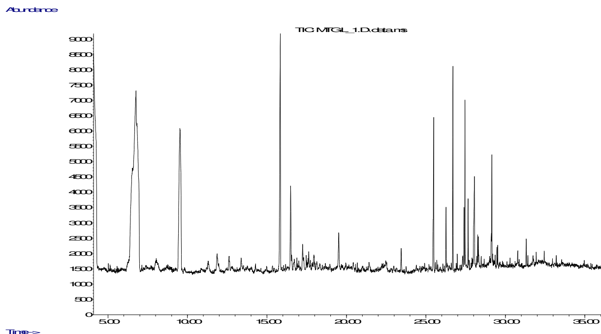
Figure 1: Gas chromatogram of the leaf essential oil of Thunbergia grandiflora [see GC conditions under experimental procedures]
