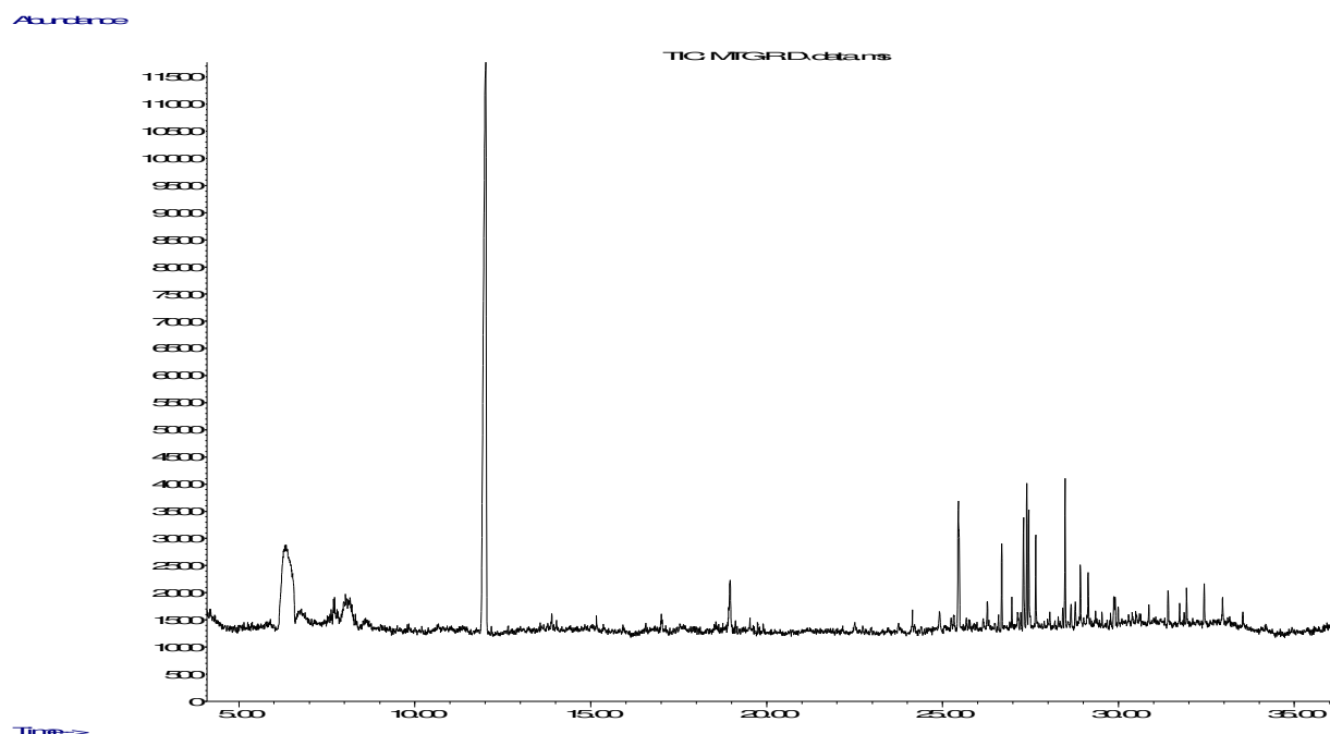
Figure 2: Gas chromatogram of the root essential oil of Thunbergia grandiflora [see GC conditions under experimental procedures]
