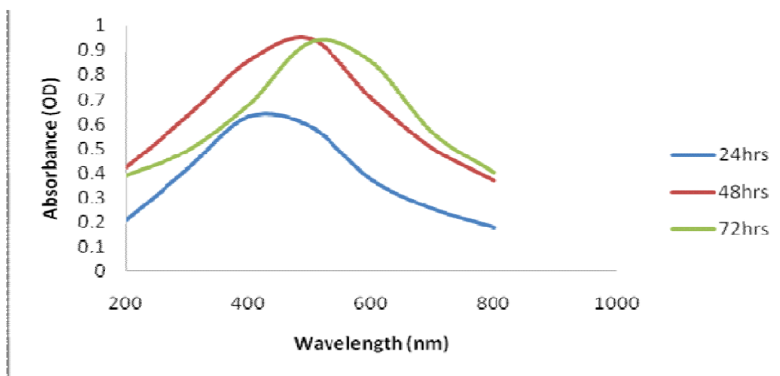
Fig. 1: UV-Vis Spectra of SNPs synthesis using Bridelia ferruginea bark extract
