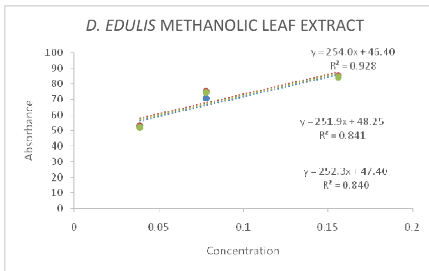
235 Figure 1b: The graph of concentration against absorbance for D. edulis methanolic leaf 236 extract.
