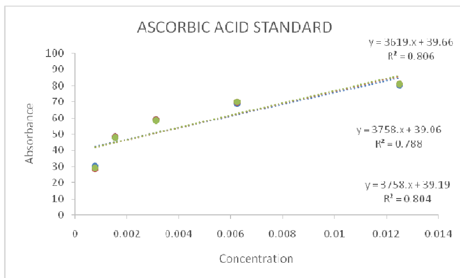
232 Figure 1a: The graph of concentration against absorbance for the standard (ascorbic 233 acid).
