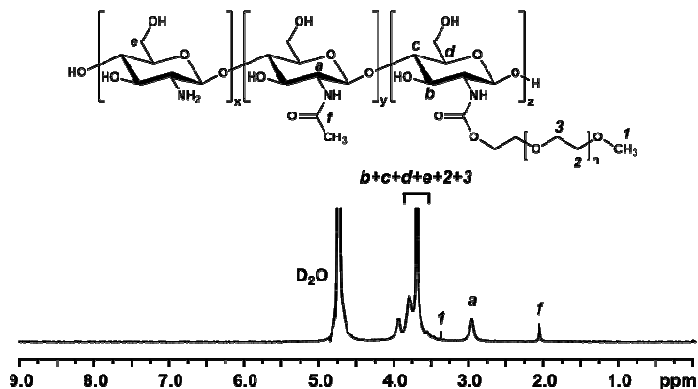
Fig. 1. ^1\text{H} NMR spectrum of mPEG-CS
