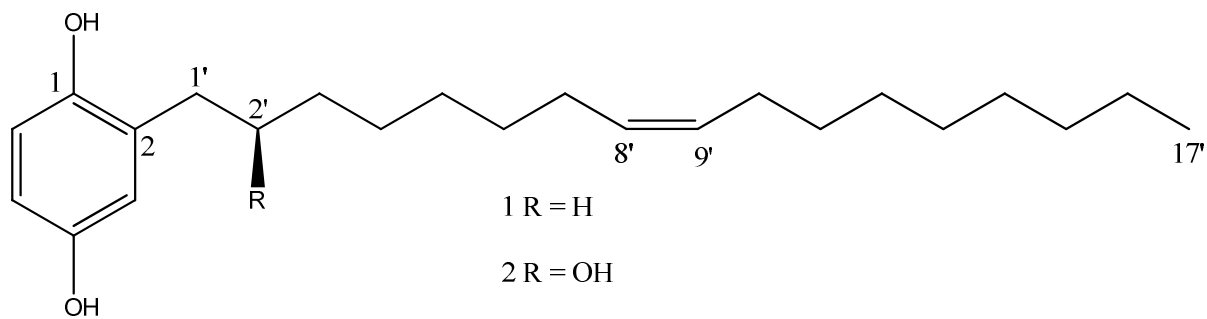
Figure 3. Cytotoxic metabolites isolated from organic fraction of Lannea welwitschii
