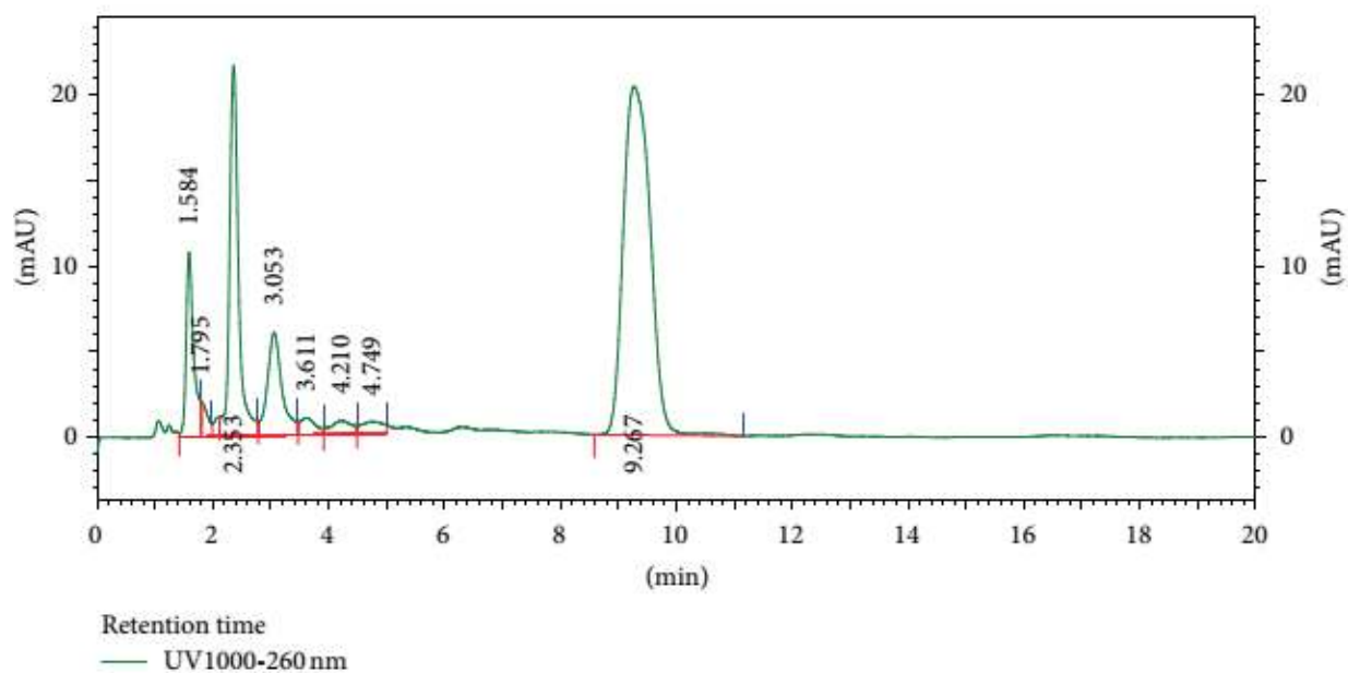
Figure 2. HPLC chromatogram (finger-printing) of methanol leaf extract of L. Welwitschii . \lambda = 254\text{nm} .
