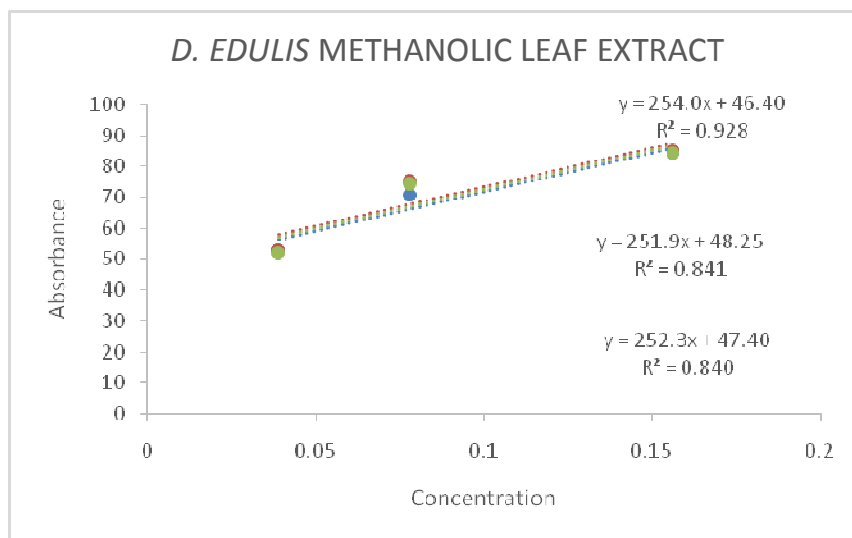
234 Figure 1b: The graph of concentration against absorbance for D. edulis methanolic leaf 235 extract.
