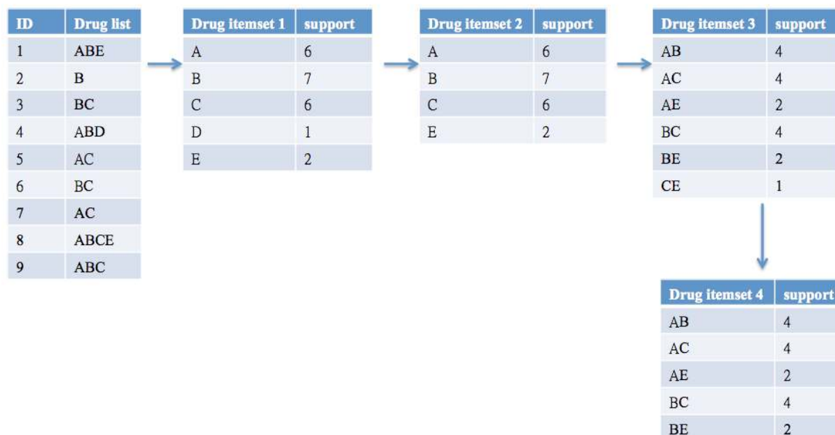
118 Fig. 5. The example of Apriori algorithm process
