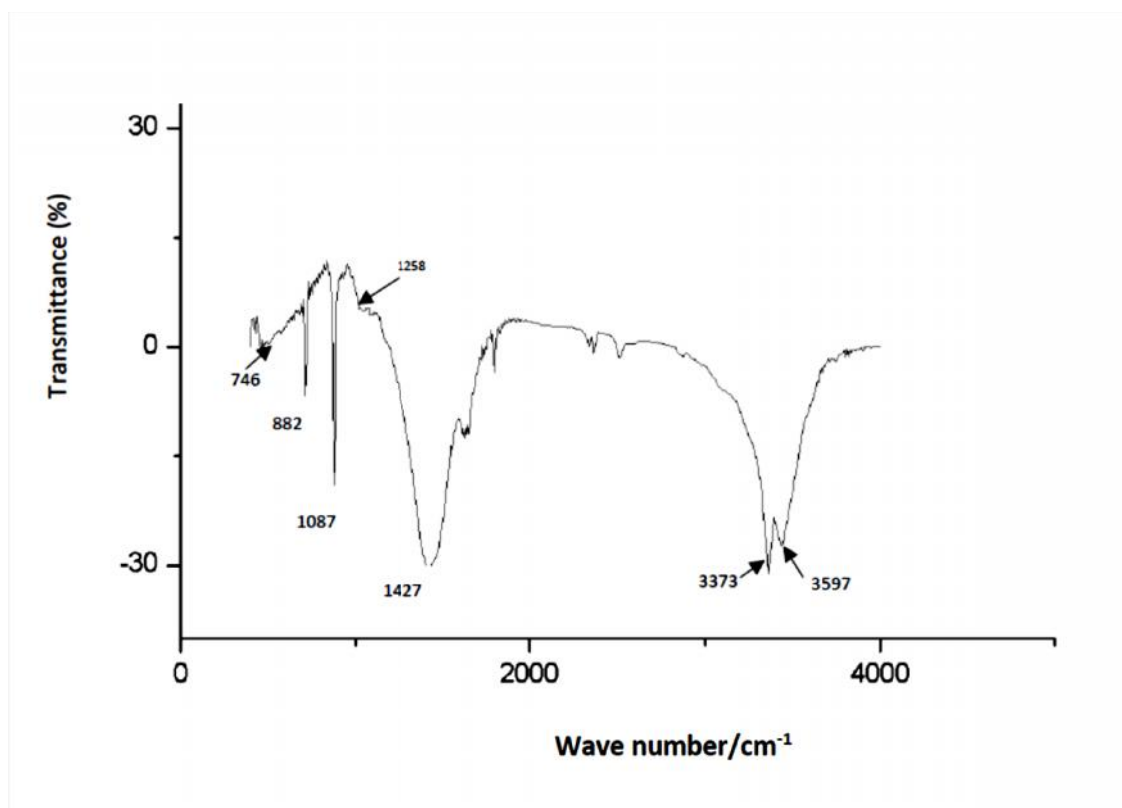
225 Figure 5: FT-IR spectrum of cisplatin encapsulated \text{CaCO}_3 nanoparticles.
