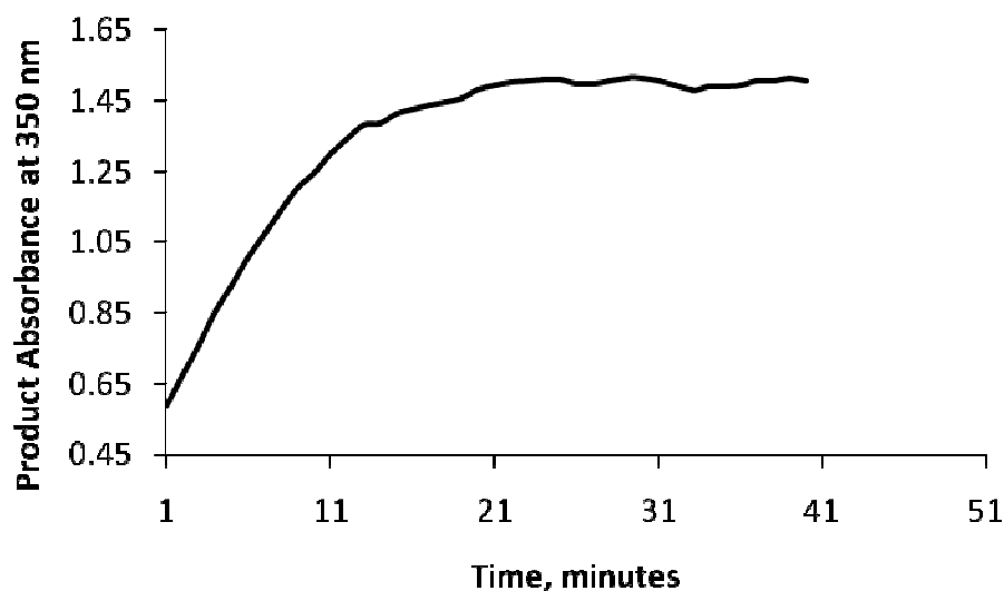
Figure 2: Time-course for the conversion of GMU. 1 mM of GMU was treated with 0.01 \mu mole of GUASE. The release of MU aglycone was monitored at 350 nm for 40 minutes.
