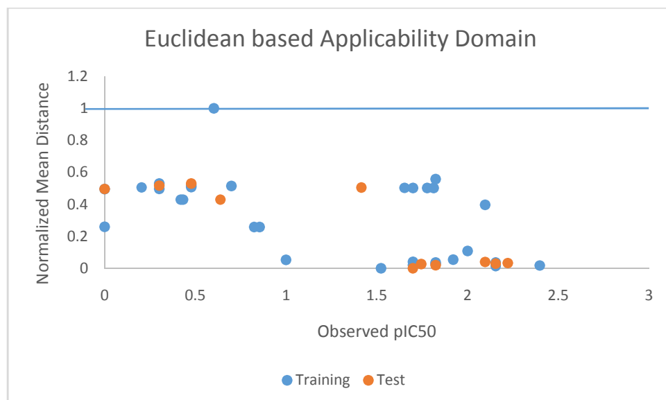
Figure 5: plot of normalized mean distance vs observed pIC50 for training and test set
