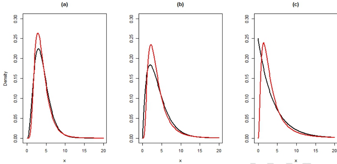
Figure 3. Comparisons of the PV_2 Distribution and the Log Normal Distribution
