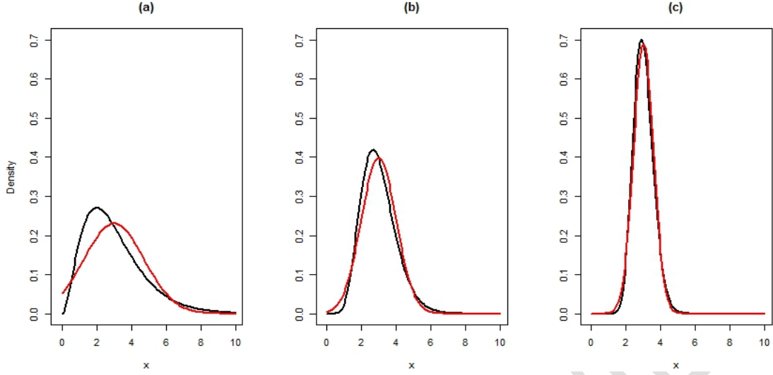
Figure 1. Comparisons of the PV_0 Distribution and the Gaussian Distribution
