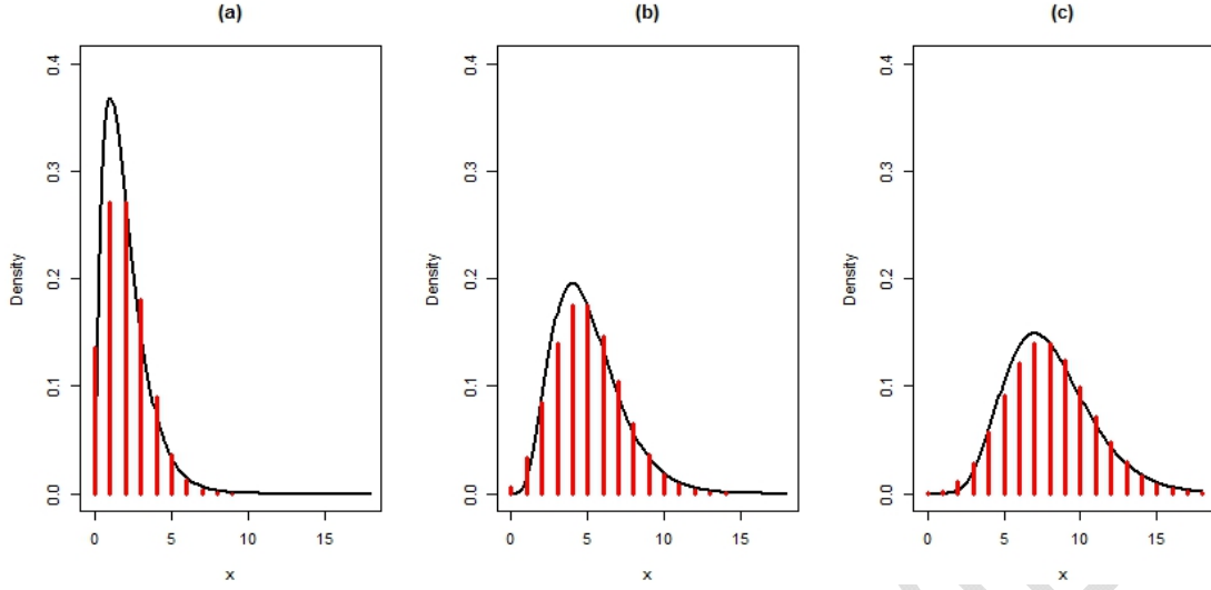
Figure 2. Comparisons of the PV_1 Distribution and the Poisson Distribution
