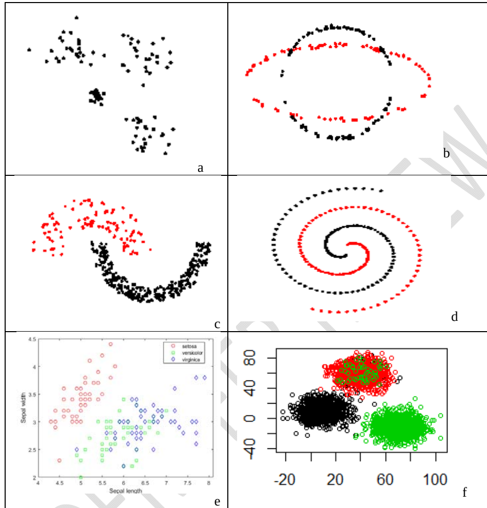
Figure 1. Data plot of synthetic and real datasets
