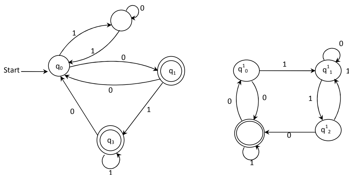
Fig. 4: Two automata B and B^1
