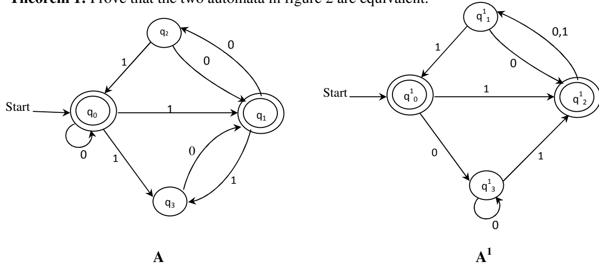
Fig. 2: Two automata A and A^1
