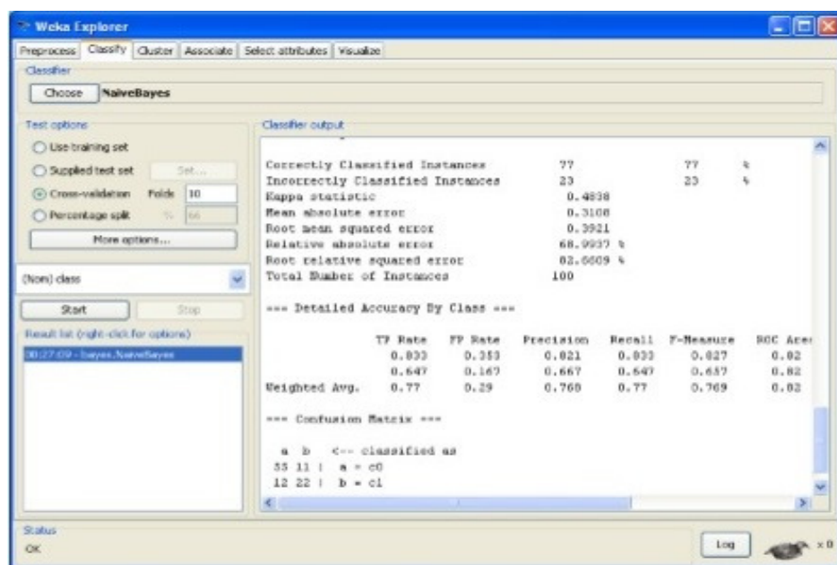
Figure 3: Naïve Bayes Result Form
