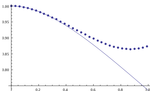
(a) Graph of exact and OHAM solutions
