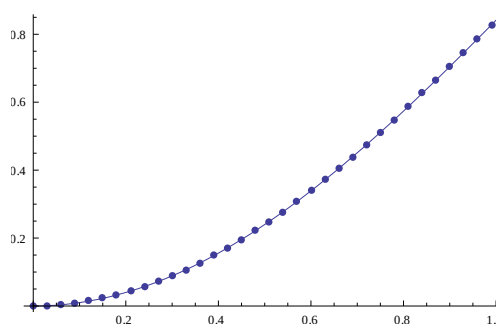
(a) Graph of exact and OHAM solutions
