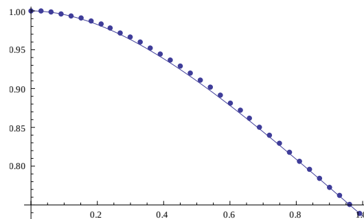
(a) Graph of exact and OHAM solutions
