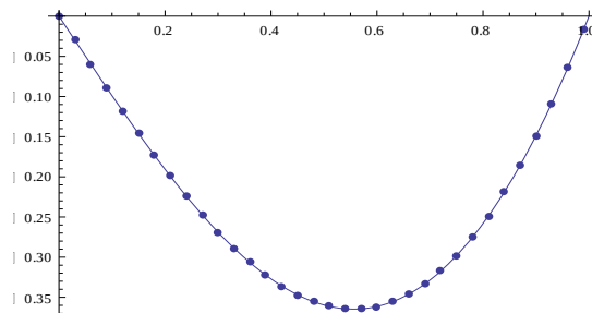
(a) Graph of exact and OHAM solutions
