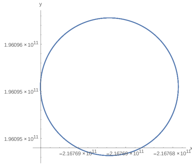
Fig.3.14: the trajectory around L_4(.8, \frac{\sqrt{3}}{2}) at \beta = .00001
