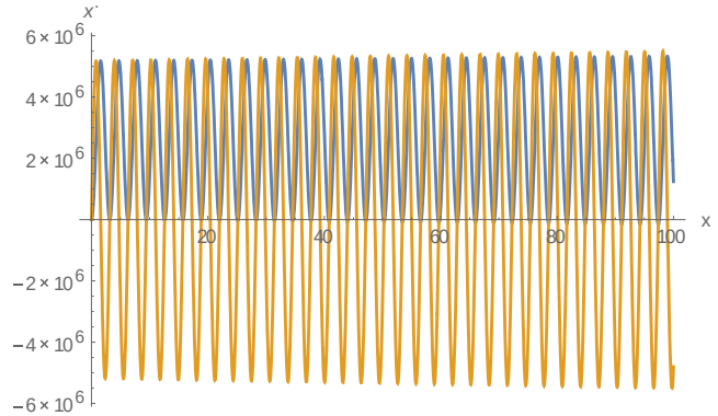
Fig.3.6.b: The phase space about L_3, \beta = -0.1 analytically
