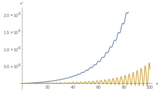
Fig.3.10.b:the phase space about L_5, \beta = -0.1
