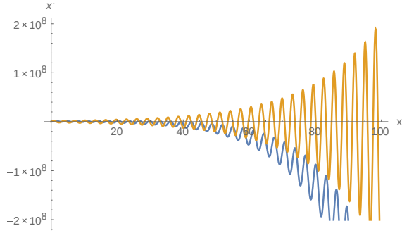
Fig.3.2.a: The phase space about L_1, \beta = -0.1 analytical
