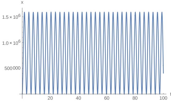
Fig.3.5.a: The analytical sol. x(t) about L_1, \beta = -0.00001
