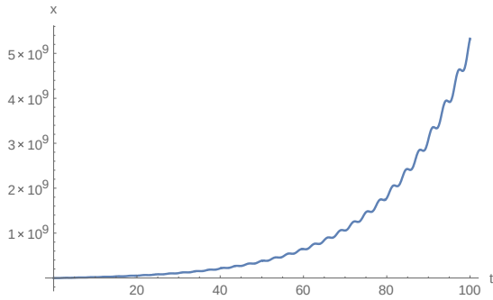
Fig.3.10.a:analytical sol. x(t) about L_5, \beta = -0.1
