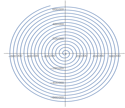
Fig.3.6.b: The phase space about L_1, \beta = -0.00001 numerical
