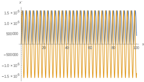
Fig.3.6.a: The phase space about L_1, \beta = -0.00001 analytical
