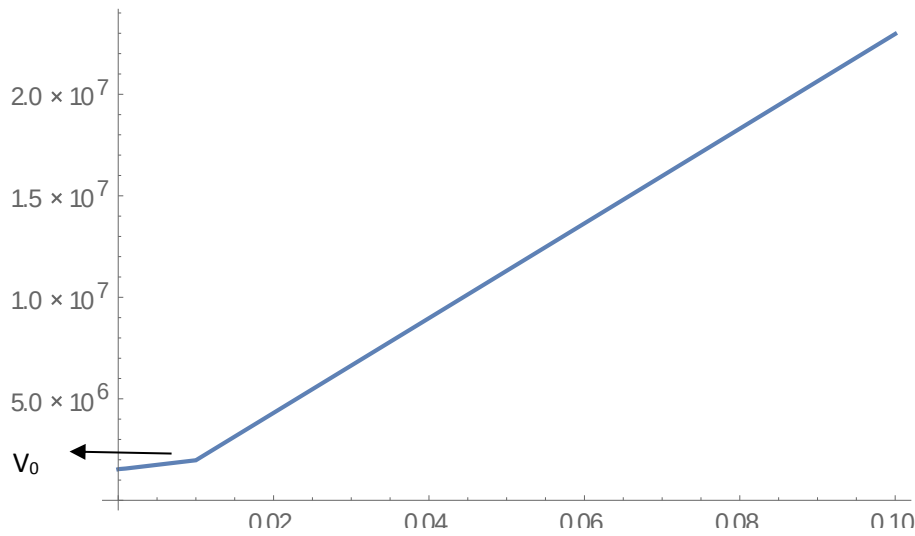
Fig.3.16: the relation between V at \beta = .1, .01, .001, .0001 at L_4(.8, \frac{\sqrt{3}}{2})
