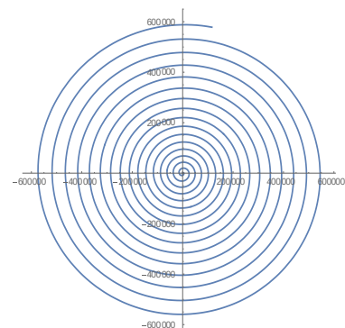
Fig.3.9.b: The phase space about L_4, \beta = -0.01 numerically
