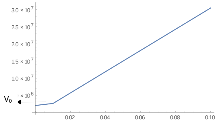
Fig.3.15: the relation between V at \beta = .1, .01, .001, .0001, .00001 at L_2(1.2, 0)
