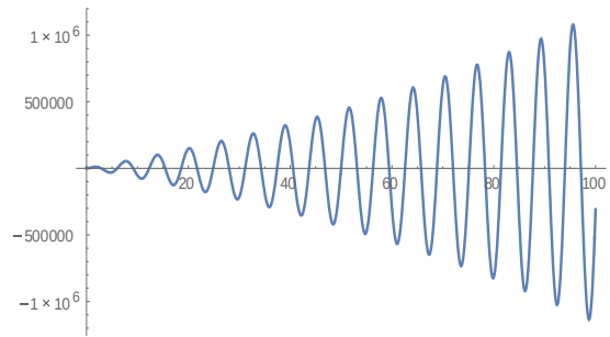
Fig.3.2.b: The phase space about L_1, \beta = -0.1 , numerical
