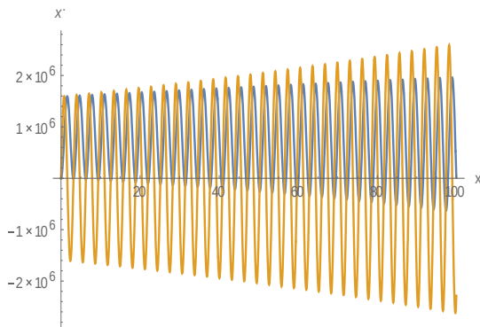
Fig.3.4.a: The phase space about L_1, \beta = -0.01 analytical
