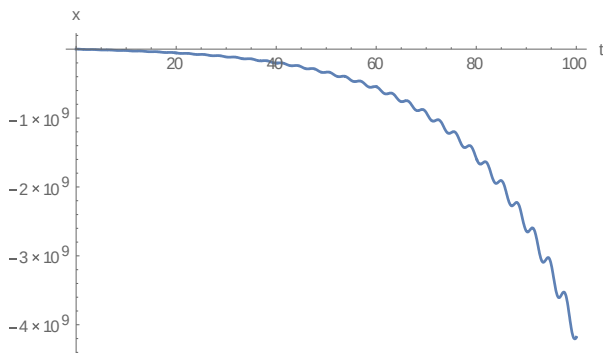
Fig.3.8.a: The analytical sol. x(t) about L_4, \beta = -0.1
