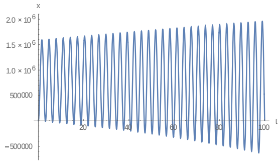
Fig.3.3.a: The analytic sol. x(t) about L_1, \beta = -0.01
