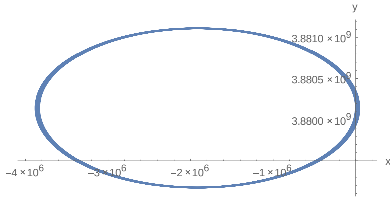
Fig.3.13: the trajectory around L_4(.8, \frac{\sqrt{3}}{2}) at \beta = .1
