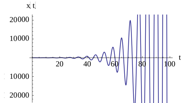
Fig.3.8.b: The numerical sol. x(t) about L_4, \beta = -0.1
