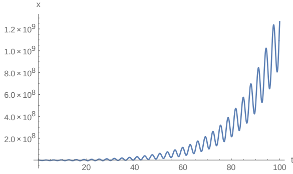
Fig.3.7.a: The analytical sol. x(t) about L_2, \beta = -0.1
