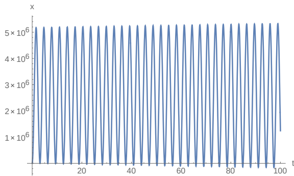
Fig.3.6.a: The analytic sol. x(t) about L_3, \beta = -0.1
