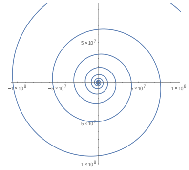
Fig.3.2.b: The phase space about L_1, \beta = -0.1 , numerical
