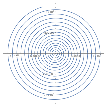
Fig.3.4.b: The phase space about L_1, \beta = -0.01 numerically
