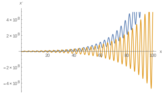
Fig.3.7.b: The phase space about L_2, \beta = -0.1 analytical
