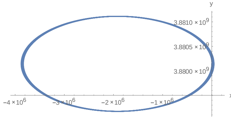
Fig.3.12: the trajectory around L_2(1.2,0) at \beta = .001
