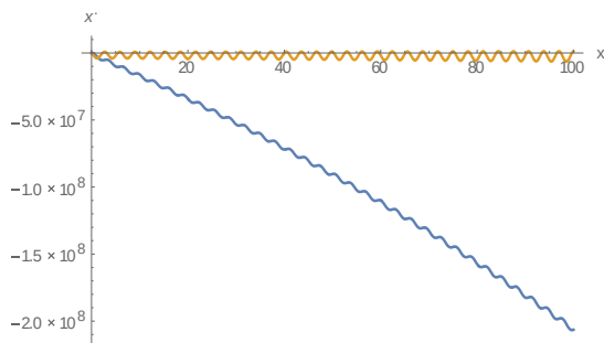
Fig.3.9.a: The phase space about L_4, \beta = -0.01 analytically
