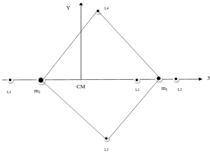
Fig.1: Libration points in 3-body problem
