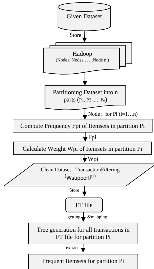
Figure 1: Framework of the Proposed FTWeightedHashT Algorithm
