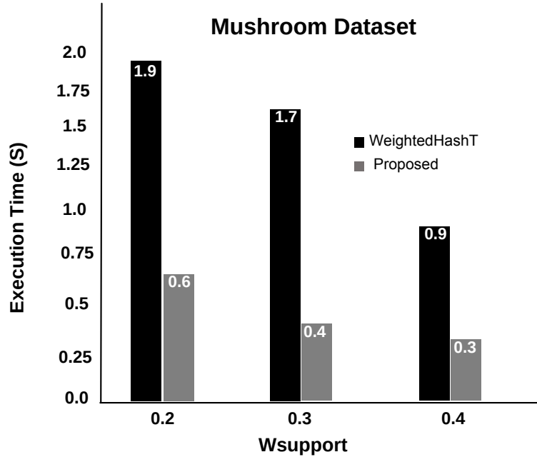
Figure 6: Execution Time comparison with Mushroom Dataset
