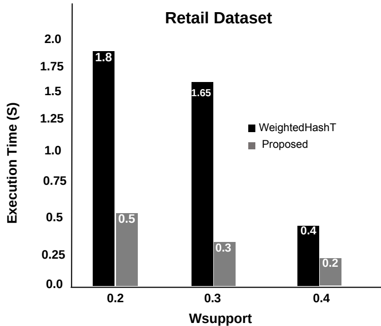
Figure 5: Execution time Comparison with Retail dataset
