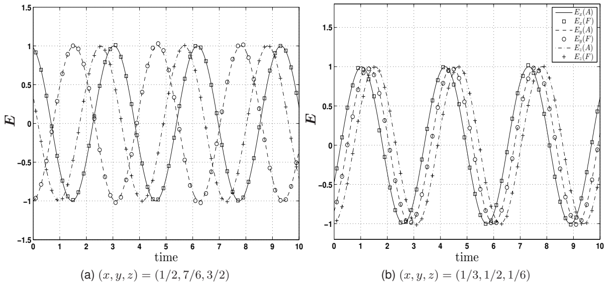
Figure 3: Time variation of the electric field for the cube with boundary-prescribed H problem.
