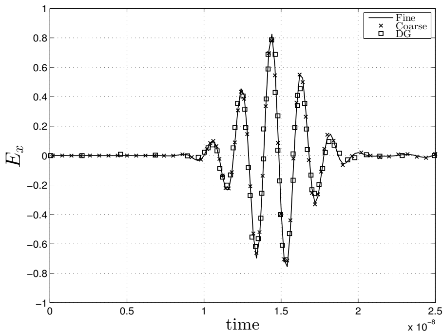
Figure 15: Scattered E_x at origin for the set of conducting spheres.
