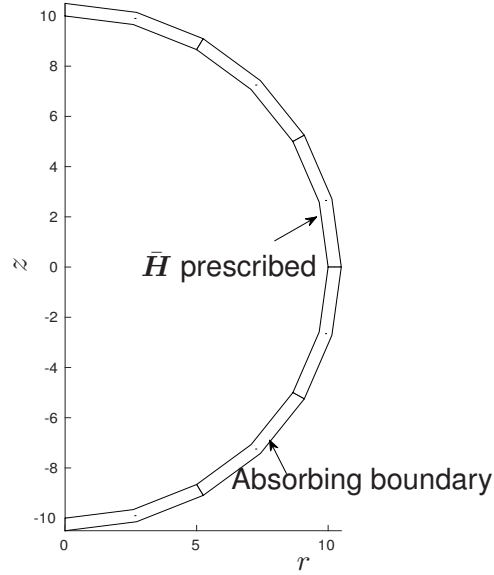
Figure 6: Mesh for the axis-symmetric radiation problem.
