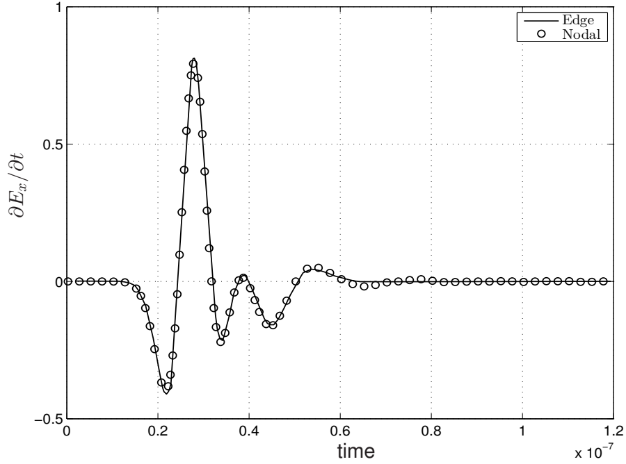
Figure 10: Time variation of \partial E_x/\partial t at (0.33, -1.03, -0.45) for the scattering from a conducting sphere example.
