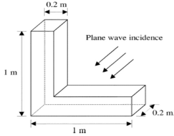
Figure 13: Geometry of the L shape domain.
