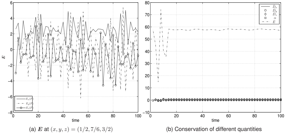
Figure 5: Bounded nature of the solution and conservation of various quantities with a very large time step for the cube with boundary-prescribed \mathbf{H} problem.
