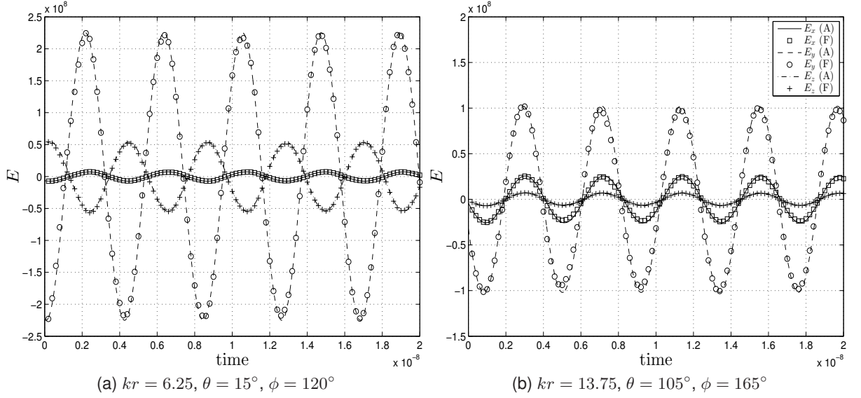
Figure 8: Time variation of the electric field for the transverse magnetic field problem.
