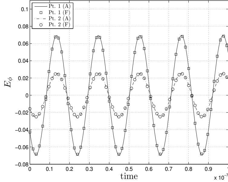
Figure 7: Time variation of electric field at Point 1 with (r, \theta) = (10.25, 45^\circ) , and Point 2 with (r, \theta) = (10.25, 165^\circ) in the axisymmetric radiation problem.
