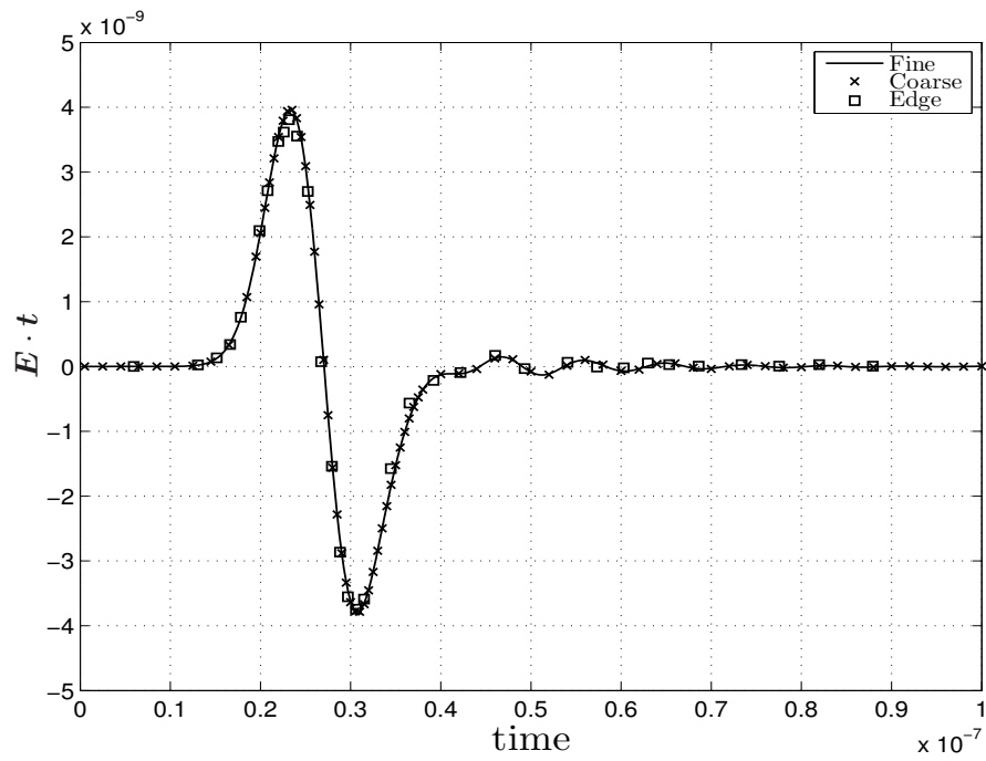
Figure 11: Time variation of E \cdot t for the scattering from a dielectric sphere example.
