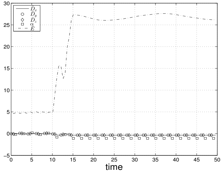
Figure 4: Conservation of different quantities for the cube with prescribed \mathbf{H} \times \mathbf{n} example.
