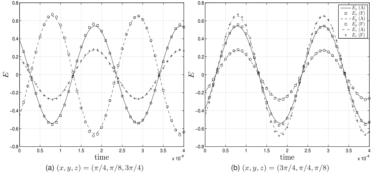
Figure 1: Time variation of the electric field for the cube with conducting walls example.
