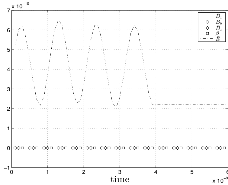
Figure 2: Conservation of various quantities in the cube with conducting walls example.
