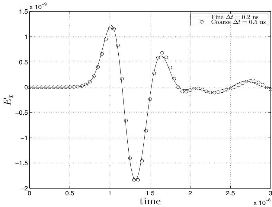
Figure 14: The variation of E_x with time at (0.55, 0.89, 0.25) for the conducting L-shaped domain problem.
