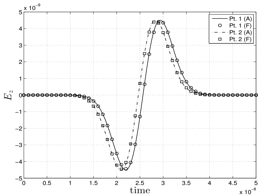
Figure 9: Time variation of the electric field at Points 1 (0.17,0.4,0.16) and 2 (0.8, 0.1, 0.6) in the scattering from an empty box problem.
