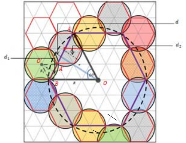
Figure 5: Overlap Difference for non-uniform Disks
