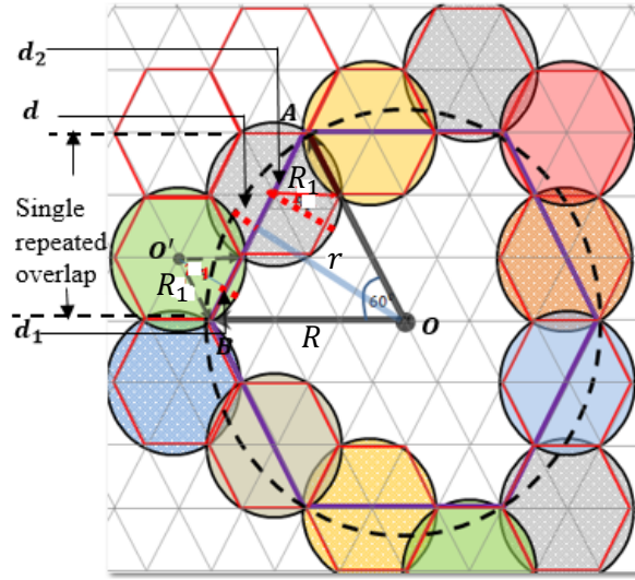
Figure 7: Area of overlap for non-uniform disks
