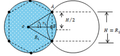
Figure 4: Overlap width for uniform disks(cell radius)
