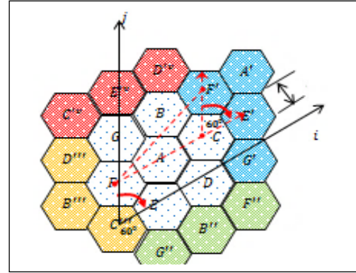
(a) N- cluster cell ( N = 7 )
