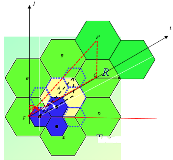
Figure 4: Generalized Frequency re-use in GSM network
