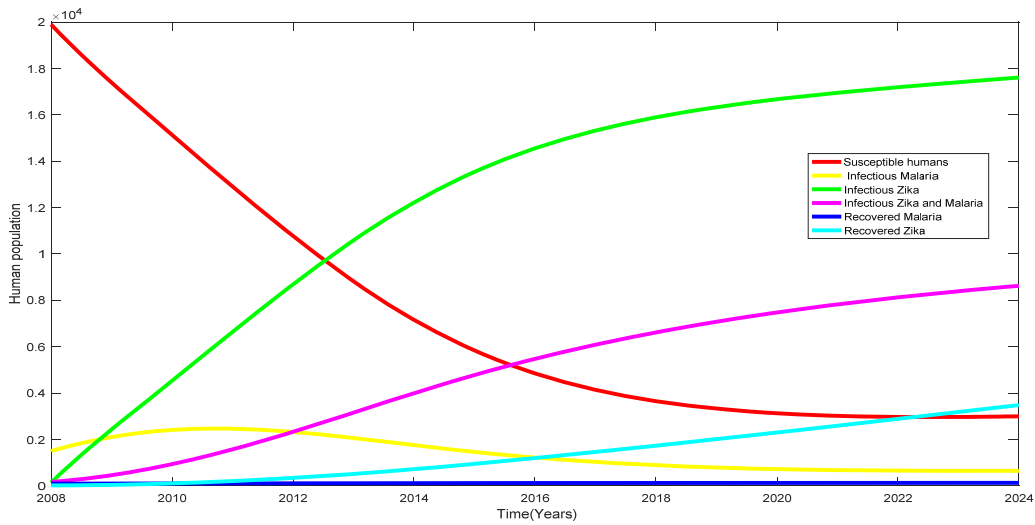
Figure 2; the plot represents the numerical solution of the model with respect to time.
