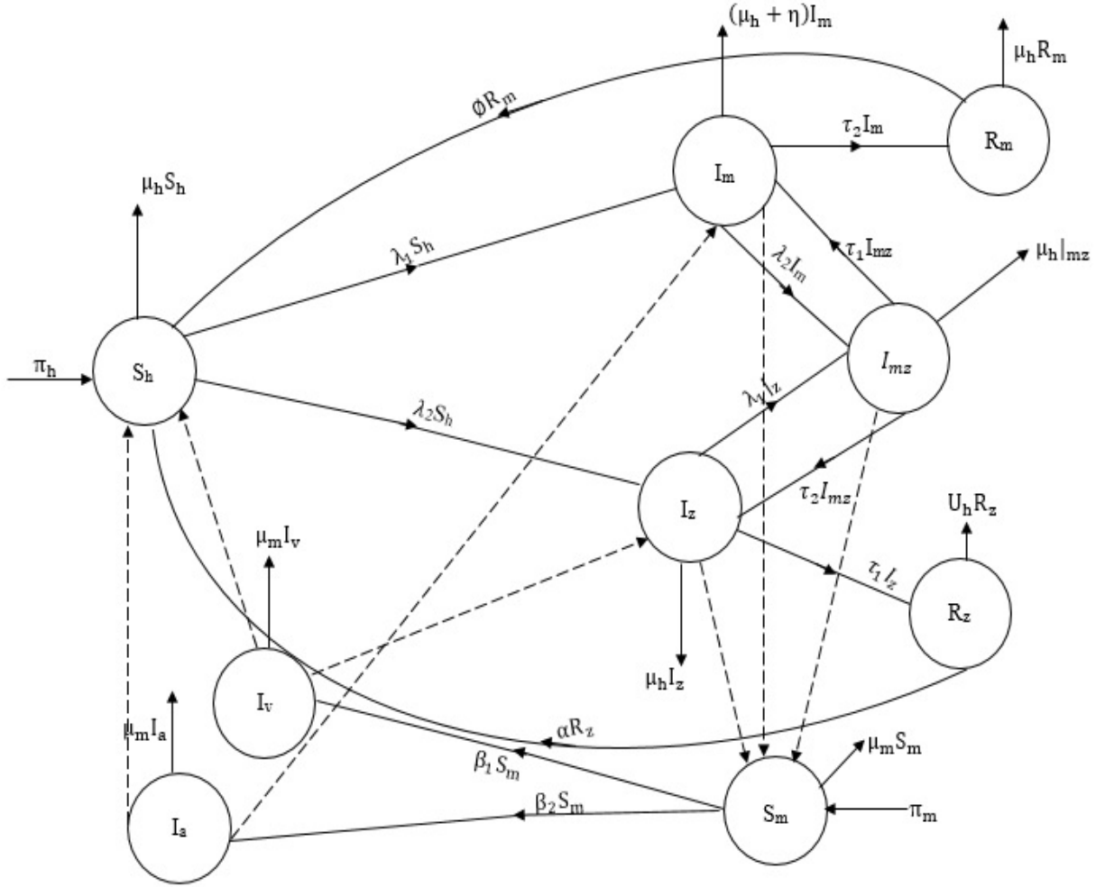
Fig 1. Flowchart of the model
