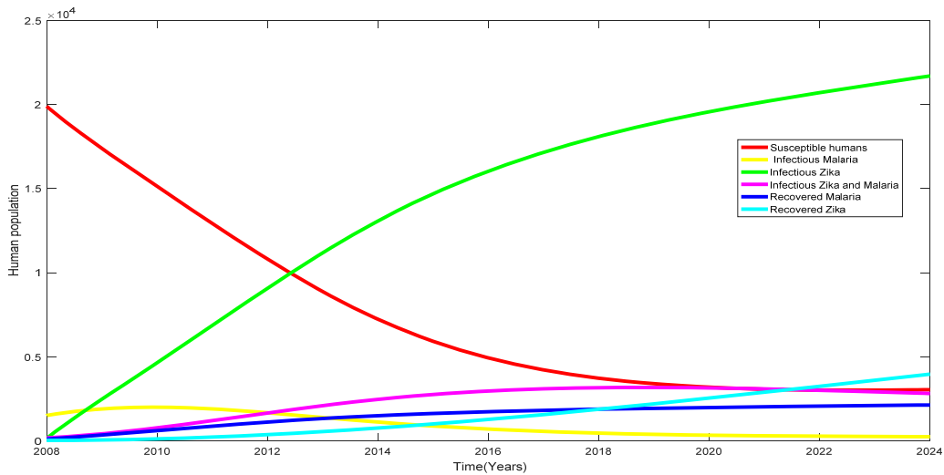
Figure 3; represents the graph of increasing the most negative sensitive index value in malaria only model.
