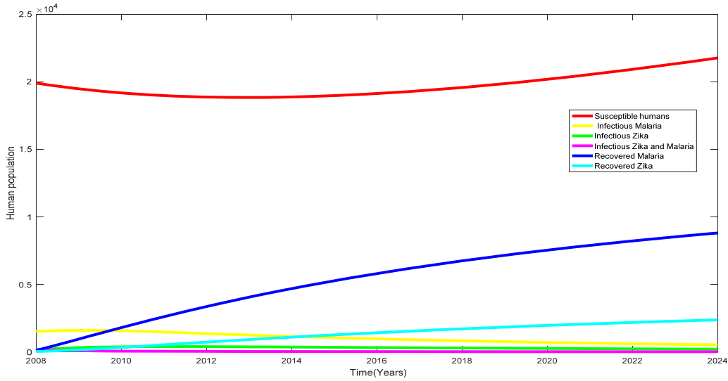
Figure 5 illustrates the plot of increasing the most negative values of both sub-models.
