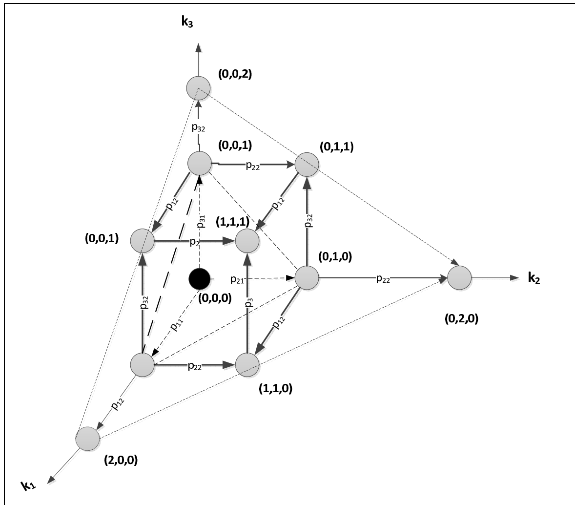
Fig. 4. Multi-dimensional Signal Flow Graph for the probability mass function of the multinomial distribution up to two generalized Bernoulli trials. A doubly-infinite number of fictitious zero nodes exist at each of the planes k_1 = -1 , k_2 = -1 and k_3 = -1 but are not shown
