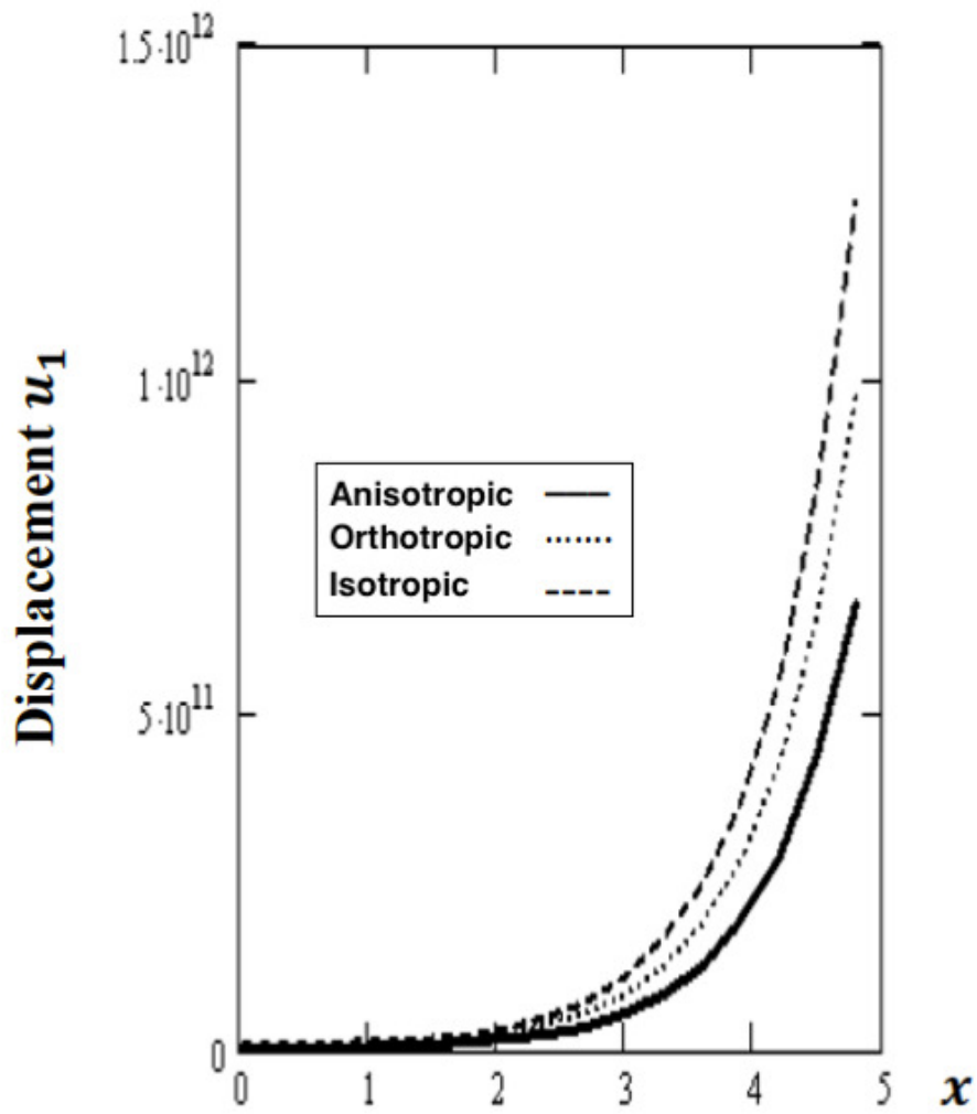
Fig. 3. Variation of the displacement u_1 with x coordinate for Anisotropic, Orthotropic and Isotropic.
