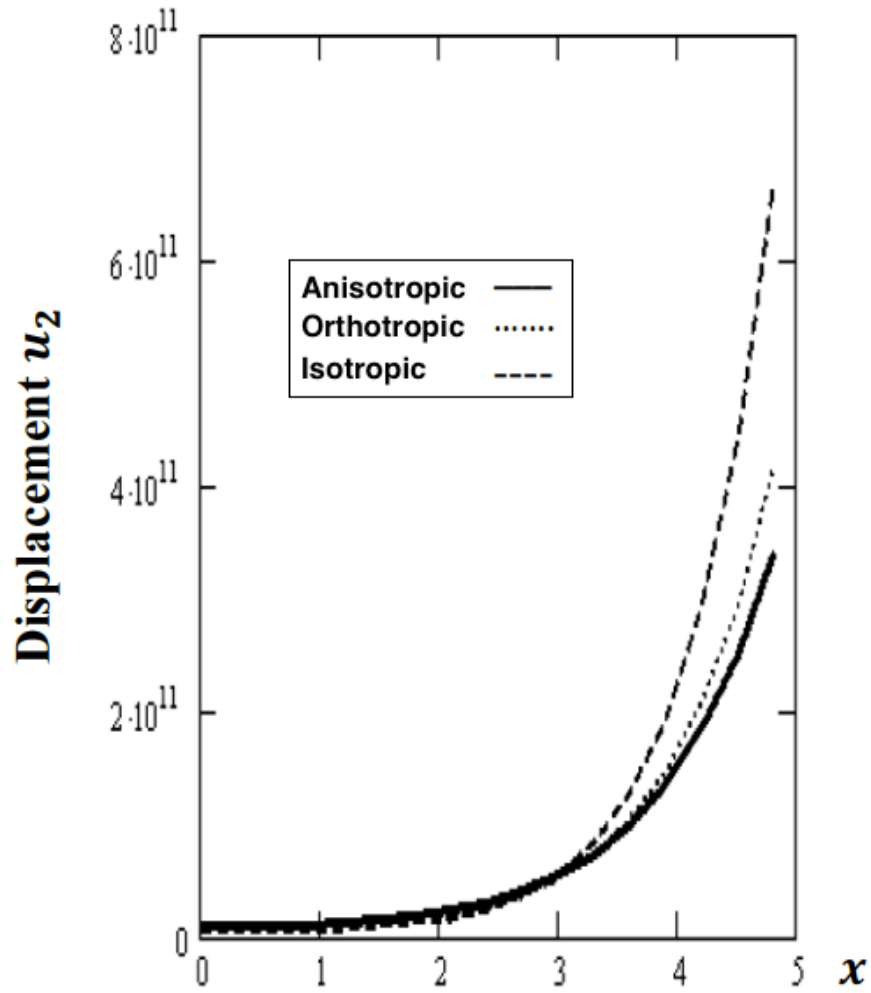
Fig. 4. Variation of the displacement u_2 with x coordinate for Anisotropic, Orthotropic and Isotropic.
