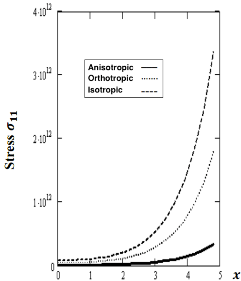
Fig. 5. Variation of the stress \sigma_{11} with x coordinate for Anisotropic, Orthotropic and Isotropic.
