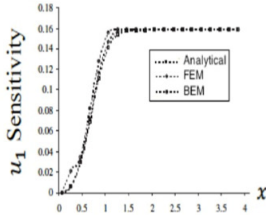
Fig. 8. Variation of the displacement u_1 sensitivity with x coordinate.
