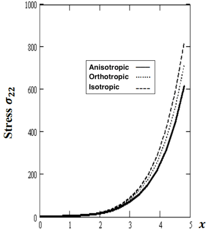
Fig. 7. Variation of the stress \sigma_{22} with x coordinate for Anisotropic, Orthotropic and Isotropic.
