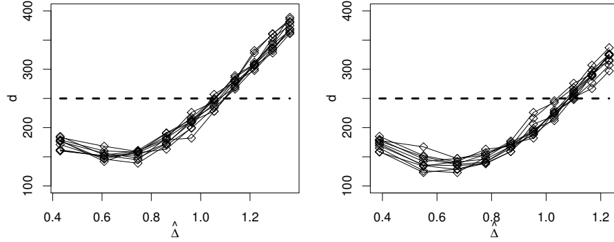
Figure 8: Relationship between \hat{\Delta} and d in the third numerical simulation (the dashed line indicates d = 250 ) (left). Relationship between \hat{\Delta} and d in the fourth numerical simulation (right).
