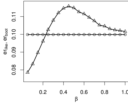
Figure 6: er_{like} ( \circ ) and er_{boot} ( \triangle ) when \beta is set to be one of \{0.05, 0.1, 0.15, \dots, 1\} .
