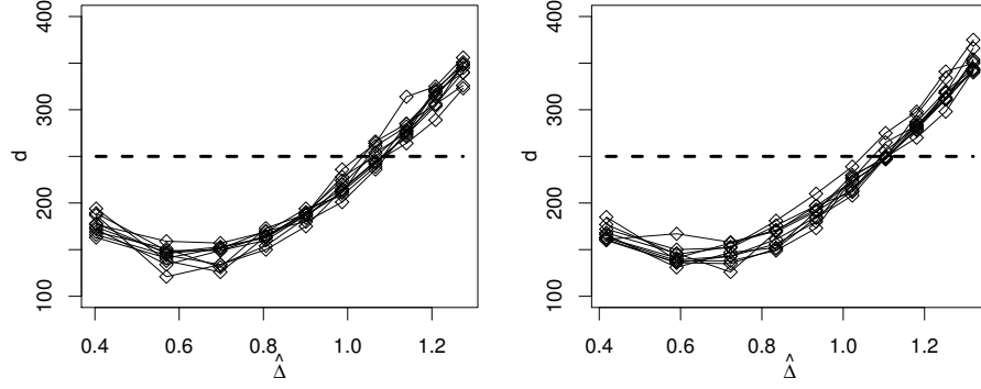
Figure 7: Relationship between \hat{\Delta} and d in the first numerical simulation (the dashed line indicates d = 250 ) (left). Relationship between \hat{\Delta} and d in the second numerical simulation (right).
