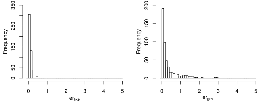
Figure 3: Histogram of values of er_{like} (left). Distribution of values of er_{gcv} (right).
