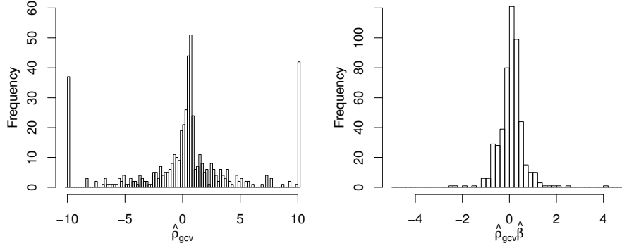
Figure 2: Histogram of the distribution of \{\hat{\rho}_{gcv}\} (left). Histogram of the distribution of \{\hat{\rho}_{gcv}\hat{\beta}\} (right).
