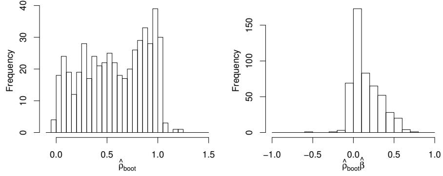
Figure 4: Histogram of \{\hat{\rho}_{boot}\} (left). Histogram of \{\hat{\rho}_{boot}\hat{\beta}\} (right).
