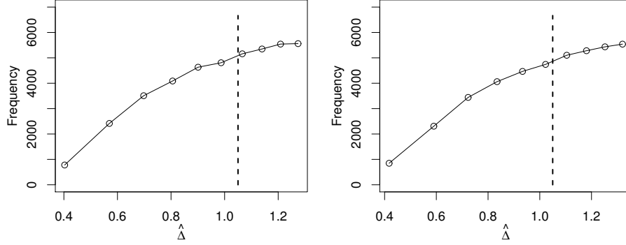
Figure 9: Left: Number of simulation data satisfying \hat{\Delta} > 1.05 from 10,000 sets of simulation data generated using the same conditions as Fig. 7(left). Right: Number of simulation data satisfying \hat{\Delta} > 1.05 from 10,000 sets of simulation data generated using the same conditions as Fig. 7(right).
