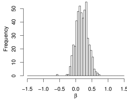
Figure 1: Histogram of \hat{\beta} obtained using 500 simulation data.
