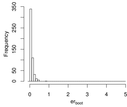
Figure 5: Histogram of values of er_{boot} .
