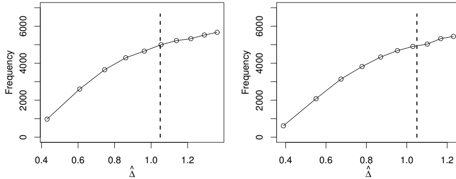
Figure 10: Left: Number of simulation data satisfying \hat{\Delta} > 1.05 from 10,000 sets of simulation data generated using the same conditions as Fig. 8(left). Right: Number of simulation data satisfying \hat{\Delta} > 1.05 from 10,000 sets of simulation data generated using the same conditions as Fig. 8(right).
