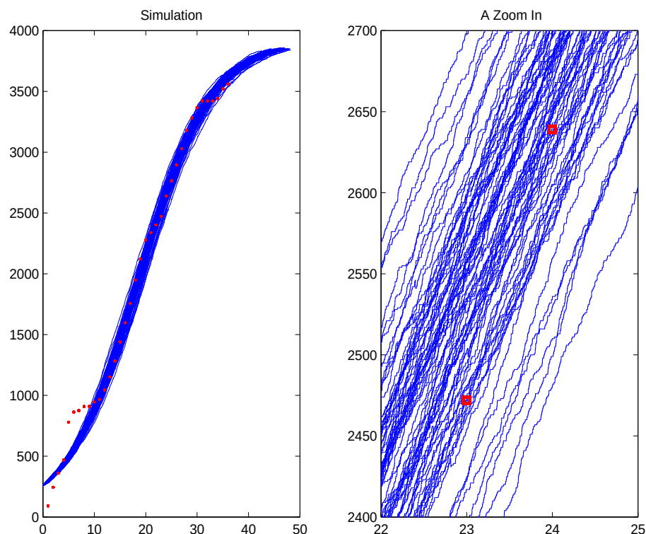
Figure 6: Simulations for the monthly samplings of snails collected in water bodies of the Tres Palmeras during 2005-2007.
