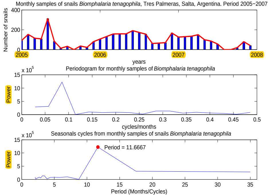
Figure 2: Top: Time series of Biomphalaria tenagophila specimens monthly sampled during 2005–2007 in the Tres Palmeras, Salta, Argentina. Middle: Periodogram of monthly samples. Bottom: Power spectrum.
