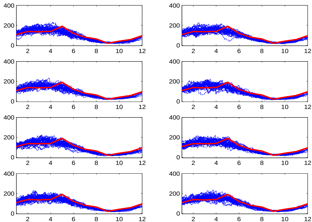
Figure 7: Monthly average of snails population dynamics during the year based on data collected for three years (2005-2007 in Tres Palmeras, period (Red line), accompanied by simulated realizations.
