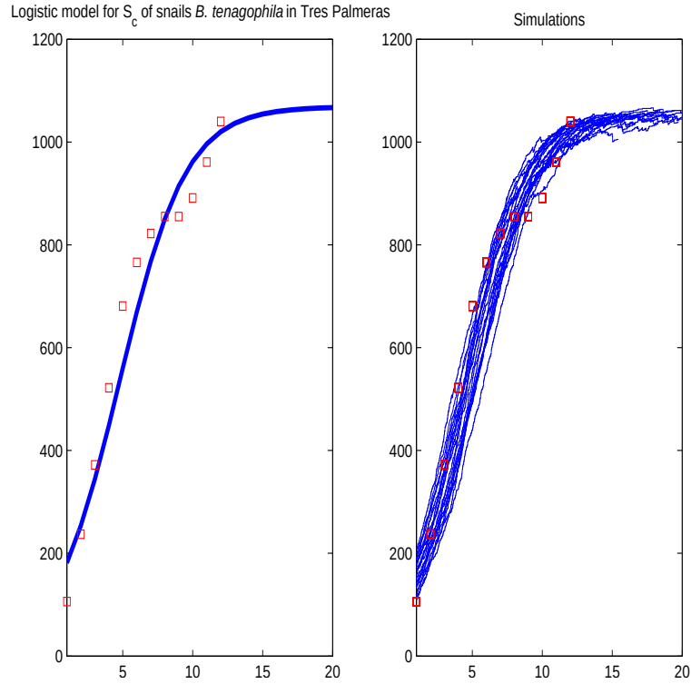
Figure 5: Left: The model (3.1) and the cumulative frequencies corresponding to the monthly data average during the three years of samplings. Right: Simulations of the logistic model (stochastic version).
