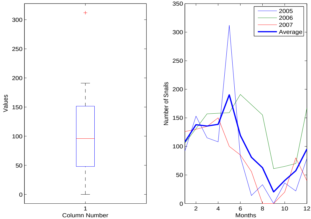
Figure 3: Left: Boxplot of Biomphalaria tenagophila monthly samplings in Tres Palmeras. Right: Dynamics of the amount of snails throughout in three years of samplings, displaying the monthly data average.
