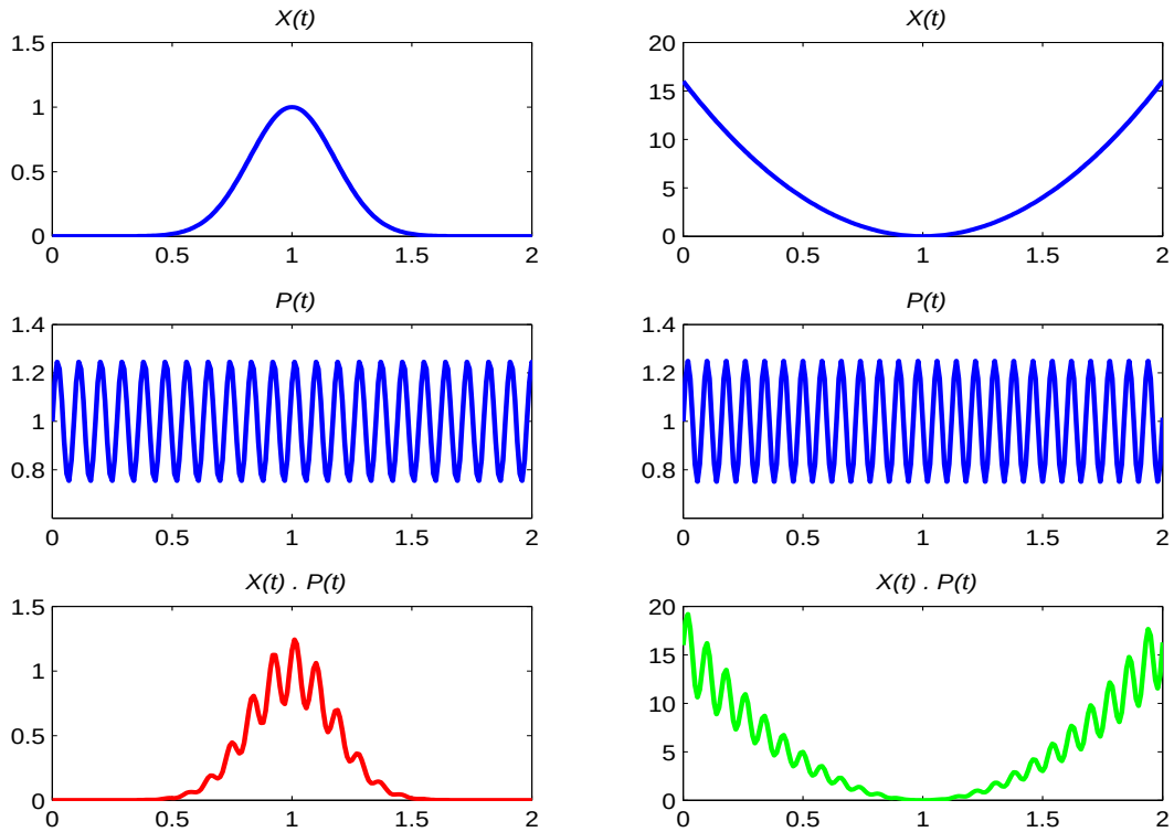
Figure 1: Examples of the effect of the waves P(t) over the functions X(t) .
