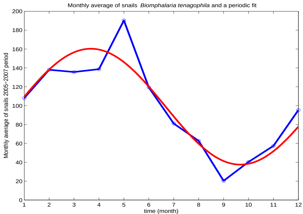
Figure 4: Monthly average of Biomphalaria tenagophila in Tres Palmeras (blue), and a periodic fit (red) for the situation analyzed.
