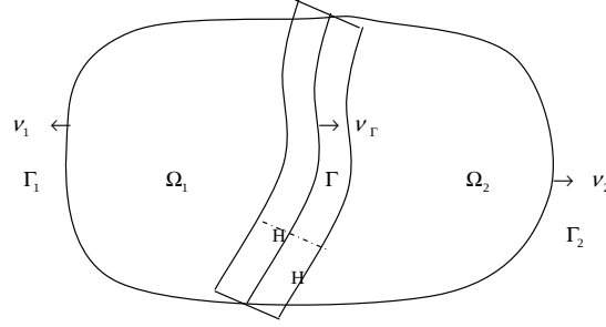
Figure 2: The strip domain G with width 2H .
