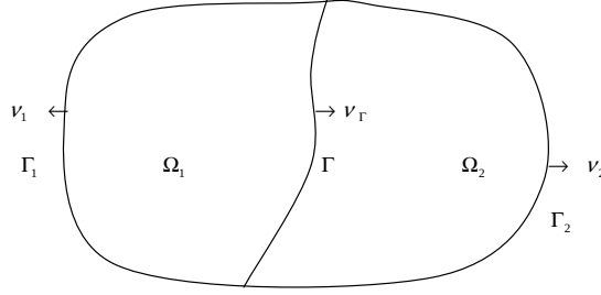
Figure 1: Subdomains \Omega_i and inter-domain boundary \Gamma .
