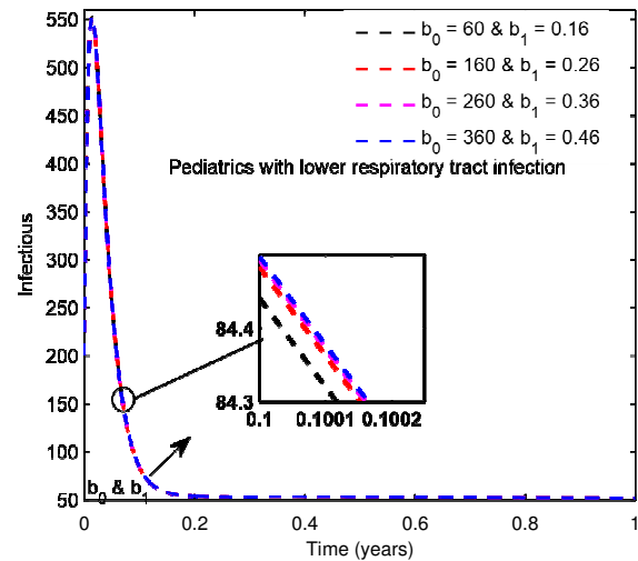
Figure 5b: Effect of b_0 and b_1 on I(t) .
