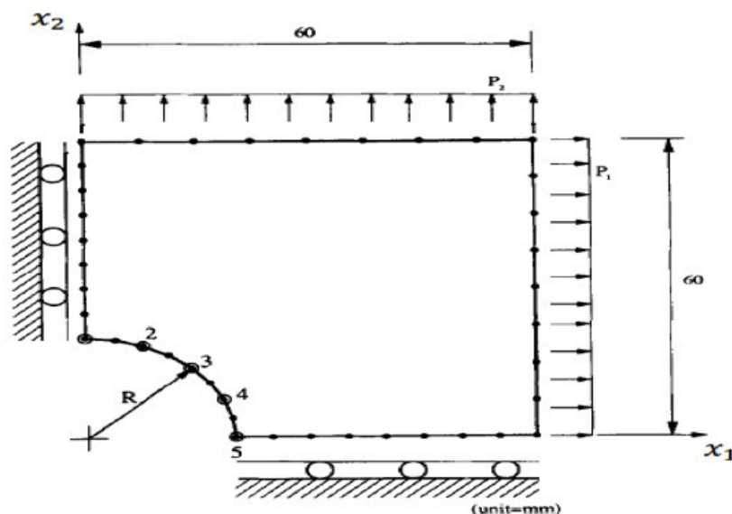
Fig. 1. Boundary element model and design variables of the plate with elliptical hole.
