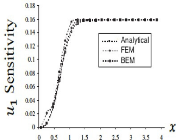
Fig. 3. Variation of the displacement u_1 Sensitivity with x coordinate.
