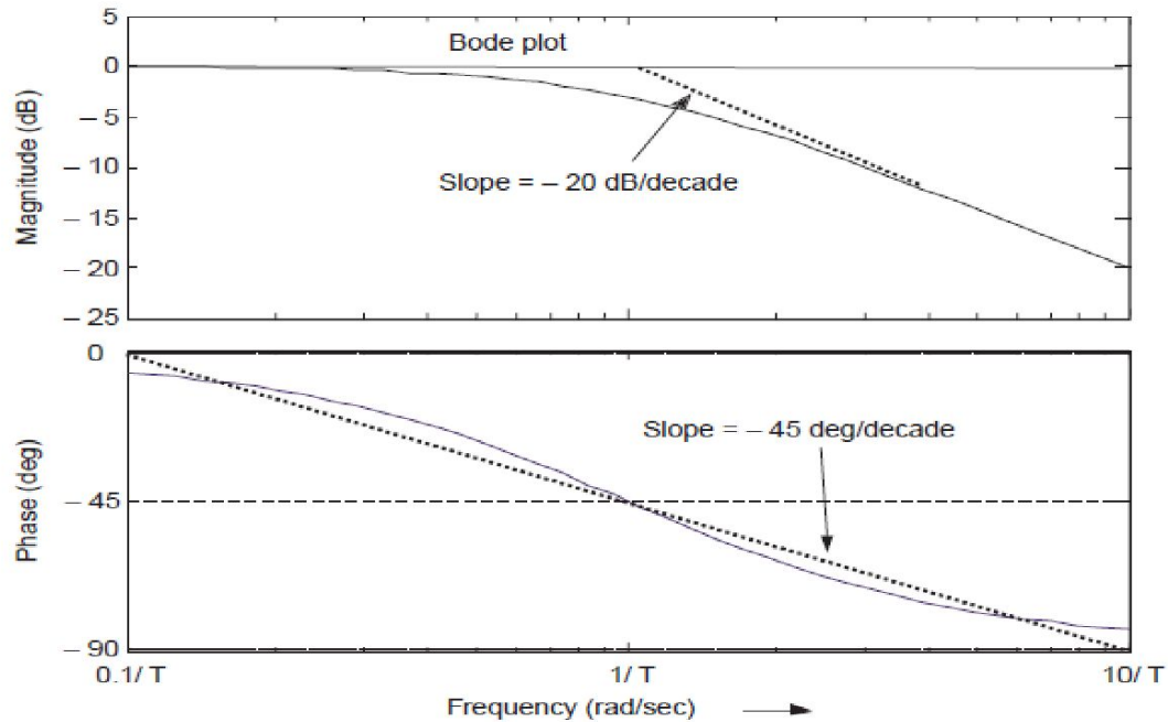
Figure 4: Bode Plot of Simple Pole, F(j\omega) = (1 + j\omega T)^{-1} [21].
