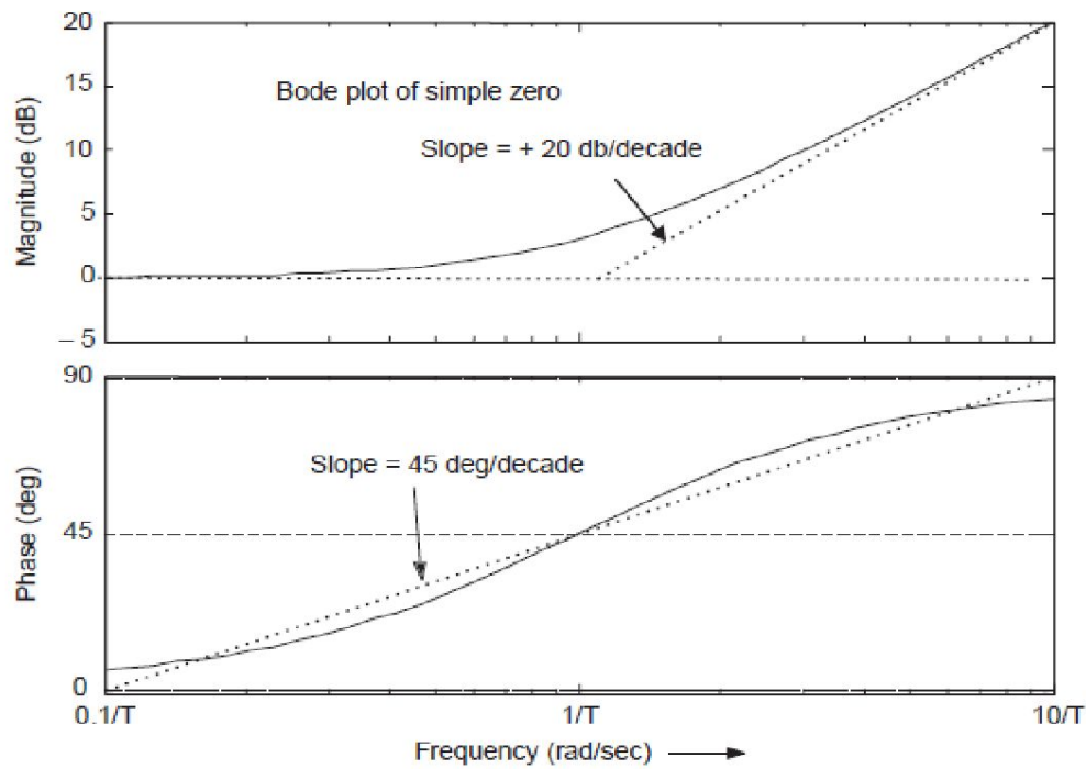
Figure 3: Bode Plot of Simple Zero, F(j\omega) = (1+j\omega t) [21].
