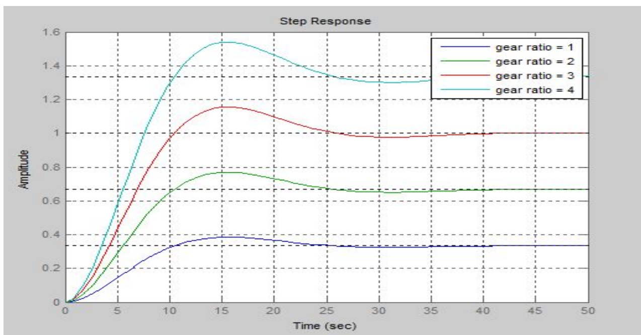
Figure 5: Step Response of the System for Different Values of Gear Ratio
