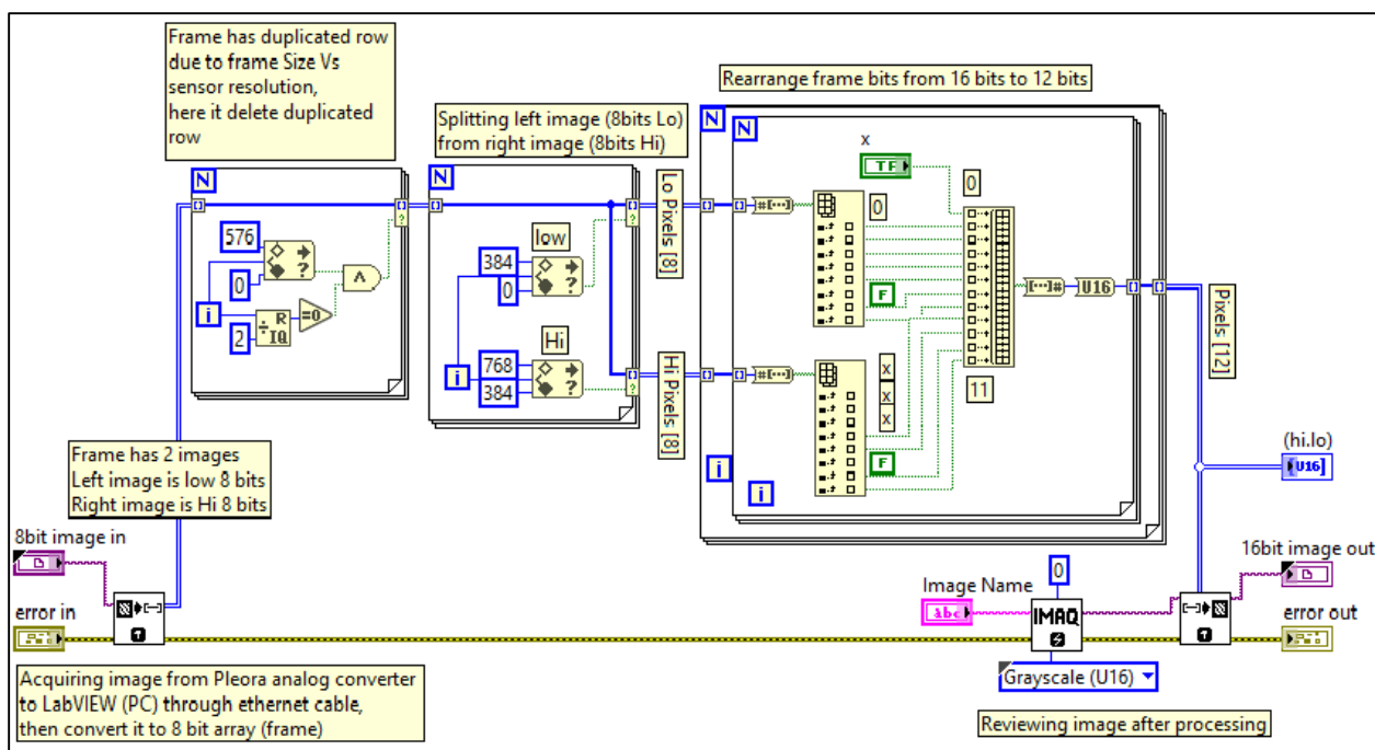
Figure 11: LabVIEW sub VI's for data aggregations and bit mapping to 12bits original form.
