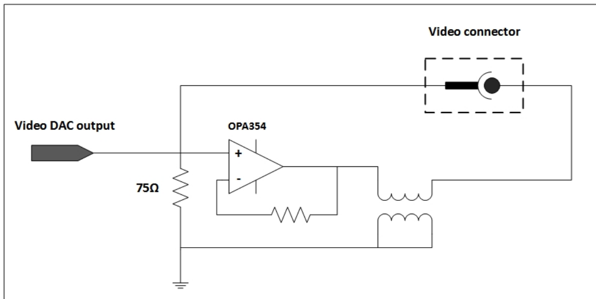
Figure 9: Impedance matching circuit
