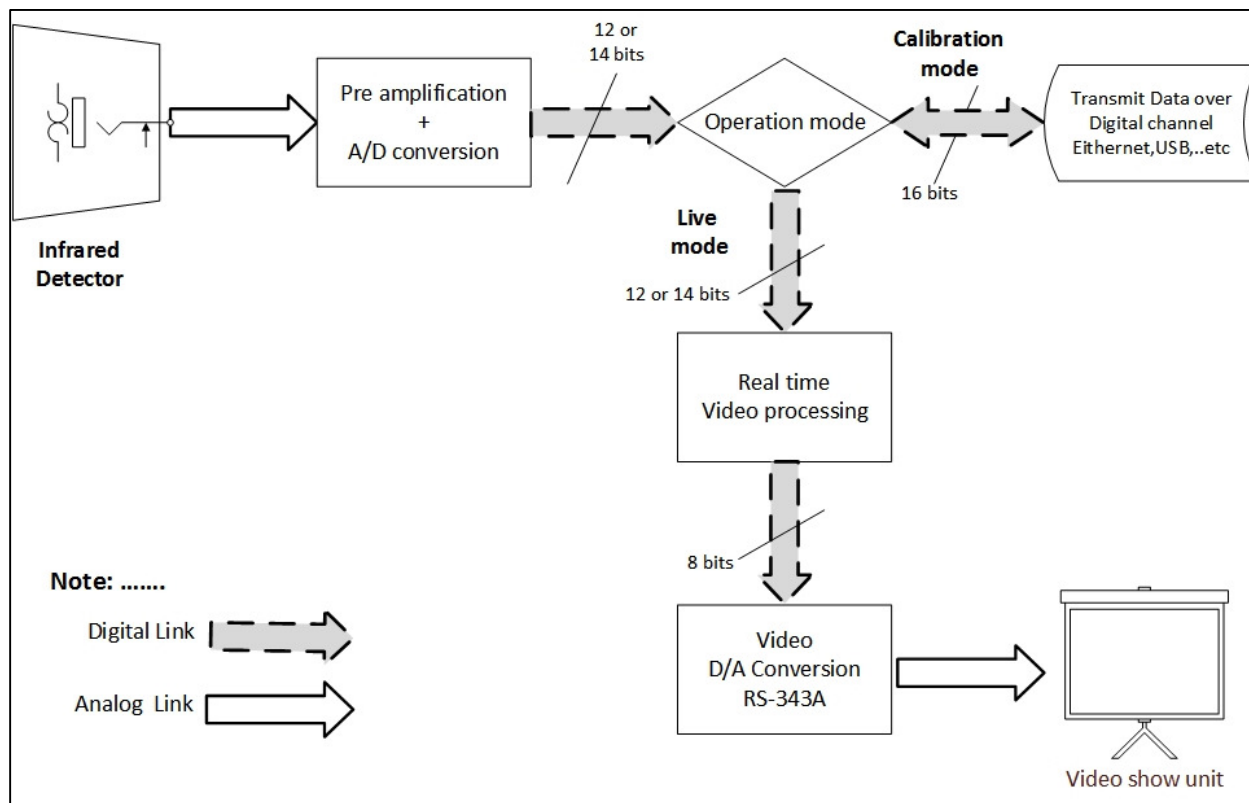
Figure 1: System basic operation modes
