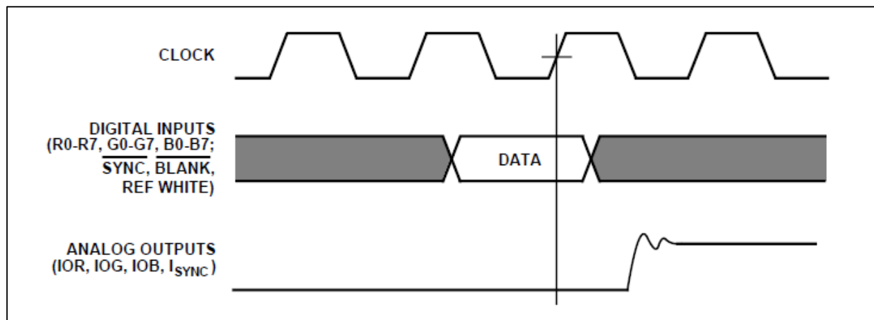
Figure 2: Video DAC Clocking Diagram
