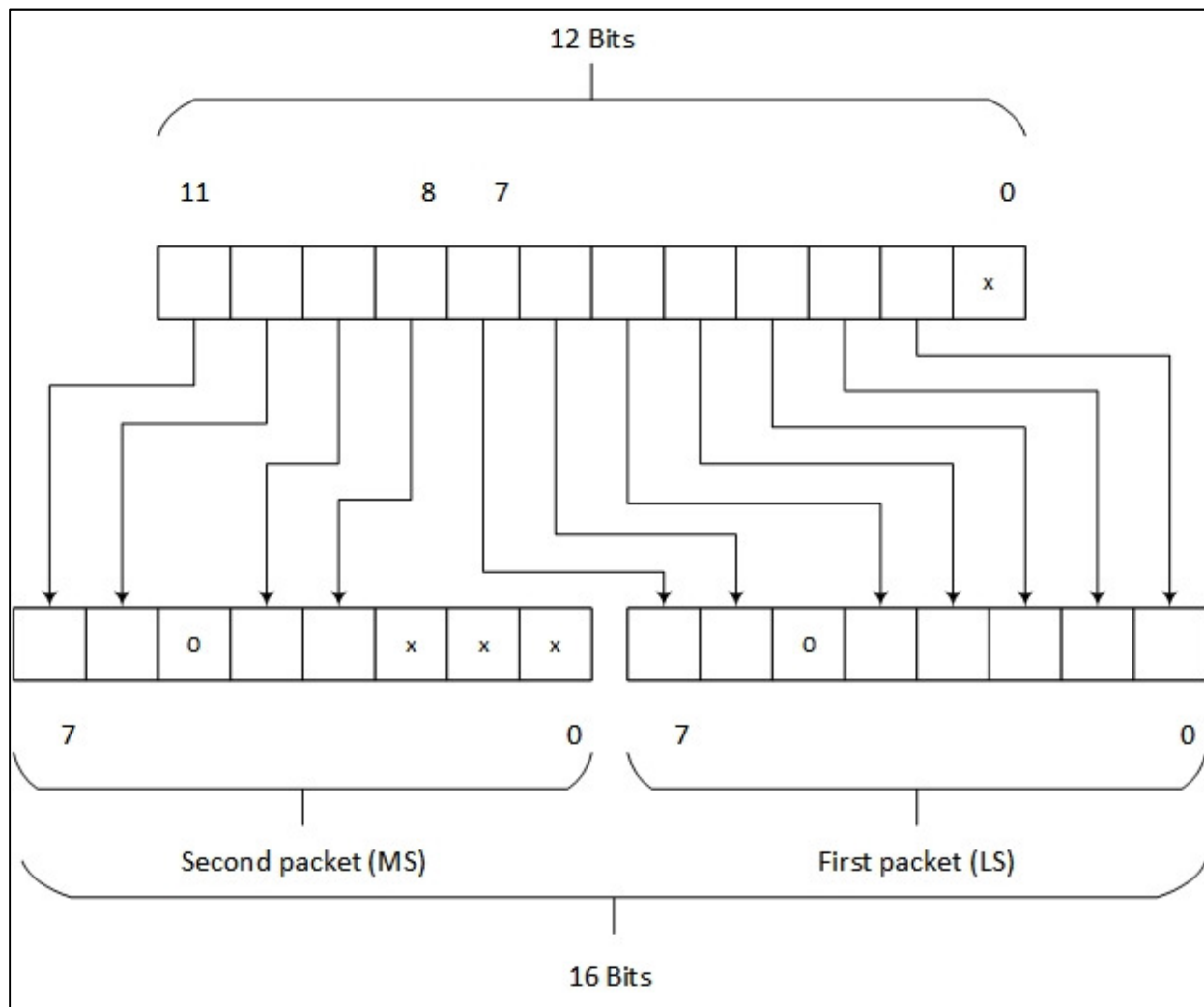
Figure 5. Two packets data manipulation
