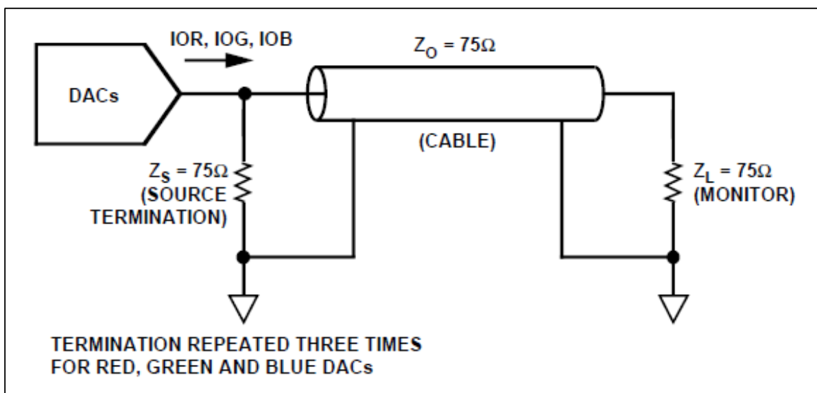
Figure 4 Impedance matching design guide for analogue video
