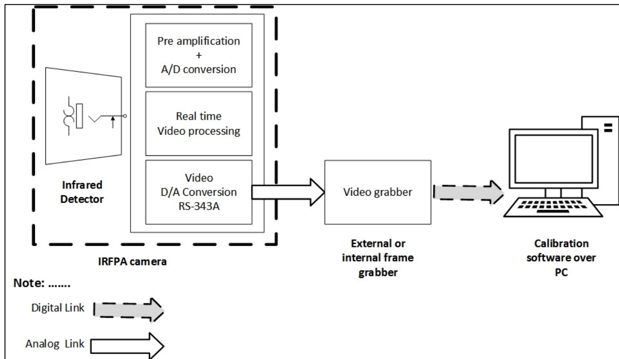
Figure 6 experiment setup which consists of IRFPA camera, calibration PC, and video frames grabber in between.
