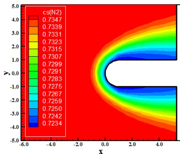
Figure 31. N 2 mass fraction contours (Park-TV).
