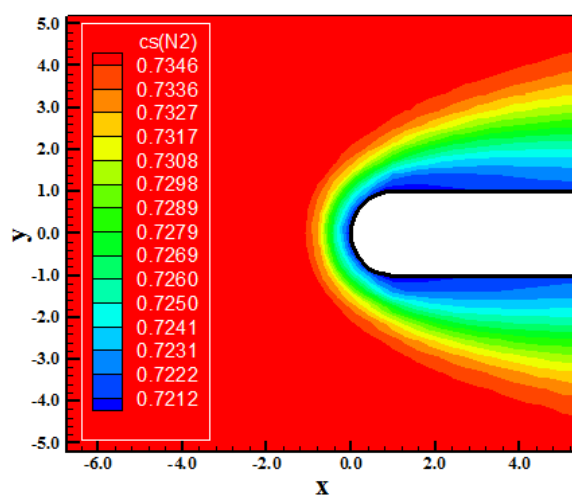
Figure 14. N_2 mass fraction contours (DK-TV).
