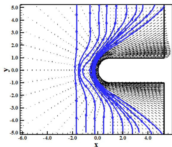
Figure 66. Induction lines (DK-TV).
