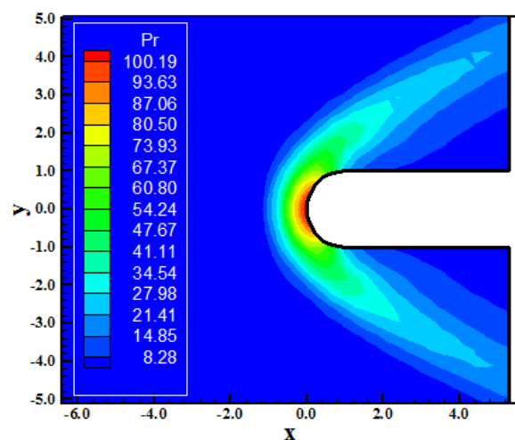
Figure 28. Pressure contours (DK-TV).
