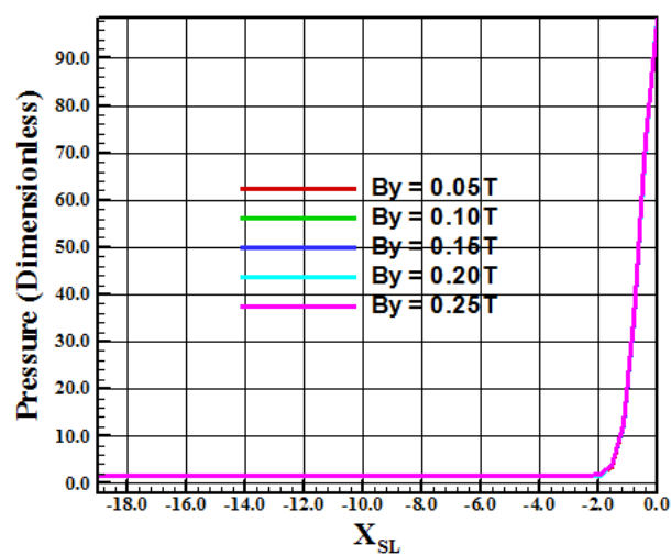
Figure 68. Pressure distribution at the stagnation line.
