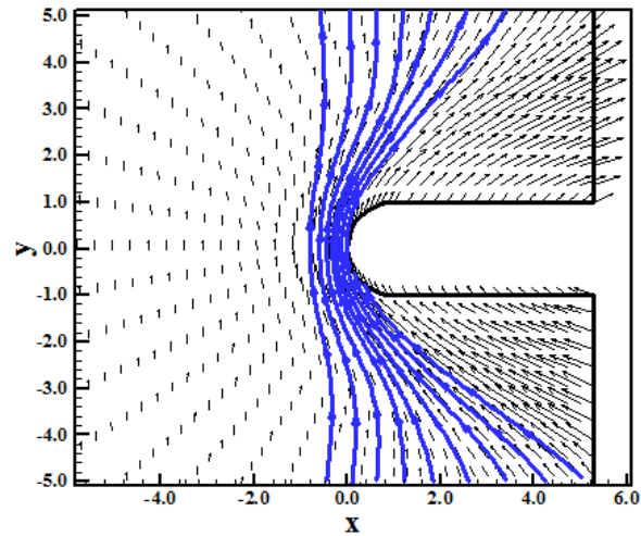
Figure 11. Induction lines (Park-MAV).
