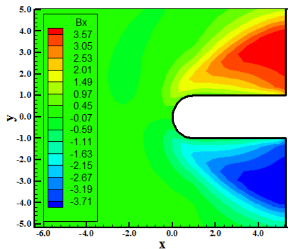
Figure 9. B x component contours (Park-MAV).
