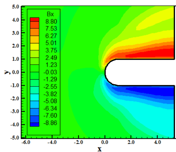
Figure 56. B_x component contours (DK-MAV).
