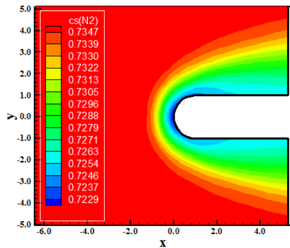
Figure 6. N_2 mass fraction contours (DK-MAV).
