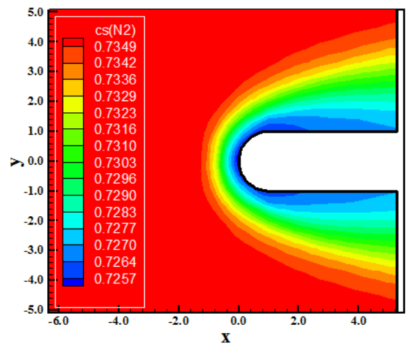
Figure 23. N_2 mass fraction contours (Park-MAV).
