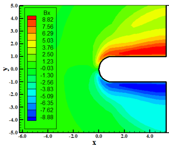
Figure 41. B_x component contours (Park-MAV).
