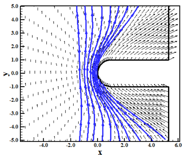
Figure 26. Induction lines (DK-MAV).
