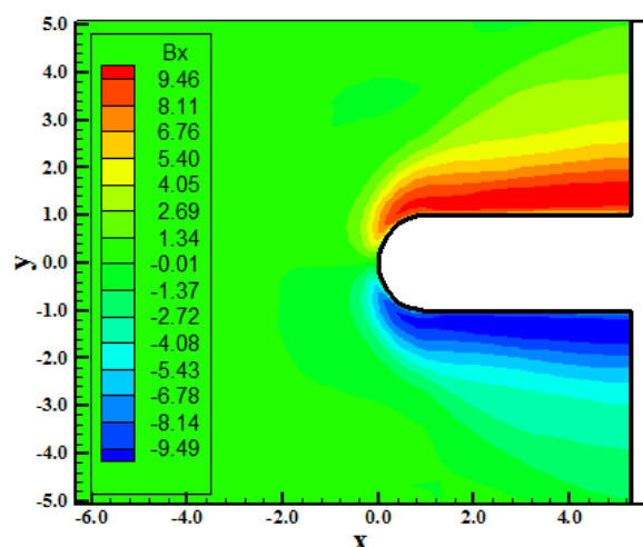
Figure 64. B_x component contours (DK-TV).
