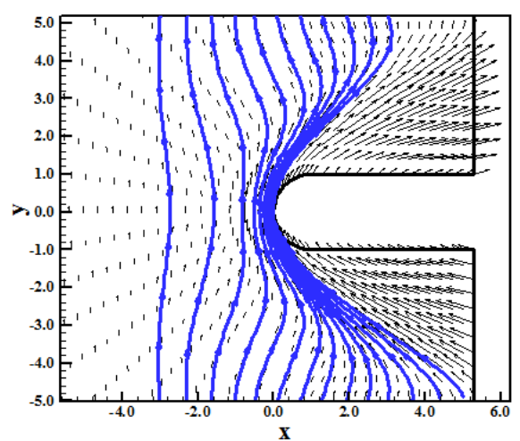
Figure 35. Induction lines (Park-TV).
