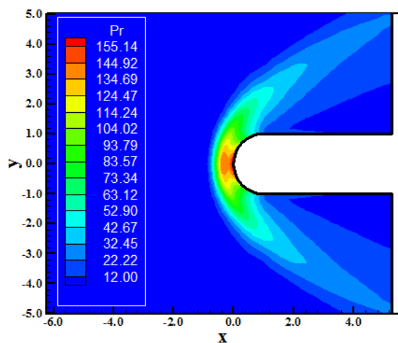
Figure 37. Pressure contours (Park-MAV).
