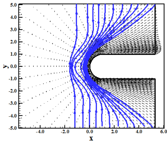
Figure 51. Induction lines (Park-TV).
