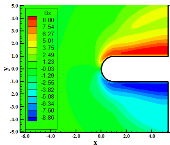
Figure 40. B_x component contours (DK-MAV).
