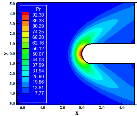
Figure 4. Pressure contours (DK-MAV).
