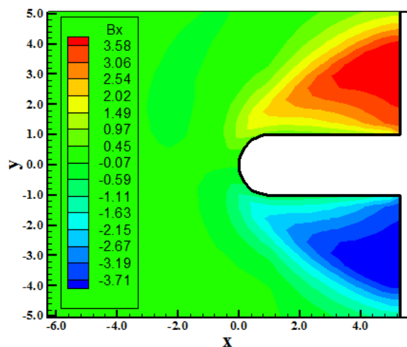
Figure 25. B_x component contours (Park-MAV).
