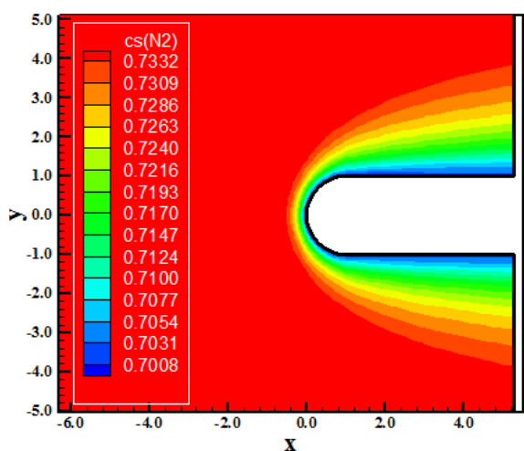
Figure 63. N_2 mass fraction contours (Park-TV).
