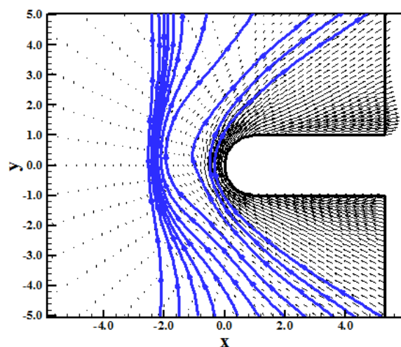
Figure 59. Induction lines (Park-MAV).
