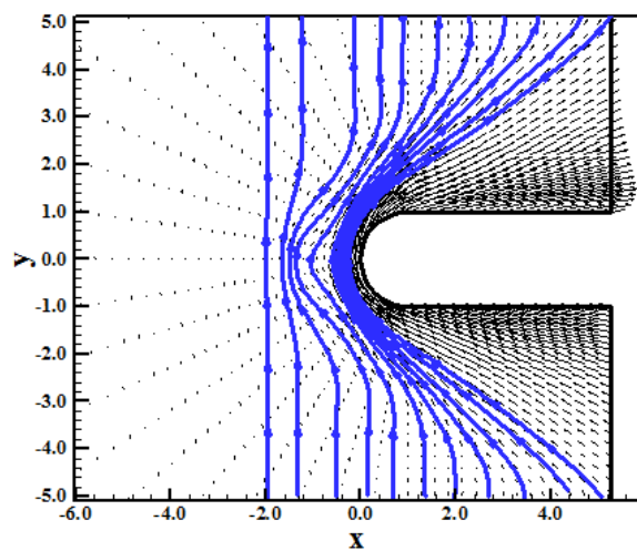
Figure 67. Induction lines (Park-TV).
