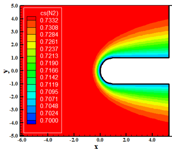
Figure 39. N_2 mass fraction contours (Park-MAV).
