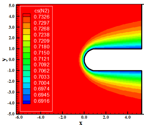
Figure 62. N_2 mass fraction contours (DK-TV).
