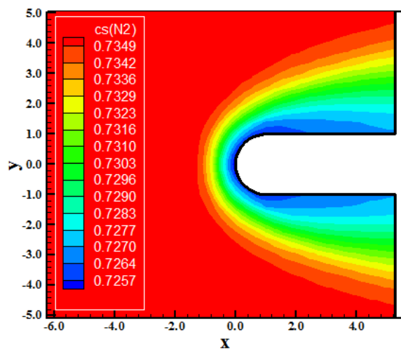
Figure 7. N 2 mass fraction contours (Park-MAV).
