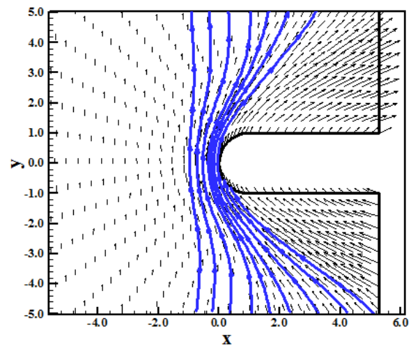
Figure 10. Induction lines (DK-MAV).
