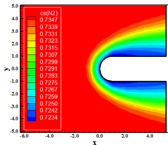
Figure 15. N_2 mass fraction contours (Park-TV).
