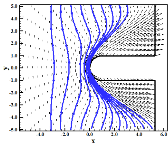
Figure 34. Induction lines (DK-TV).
