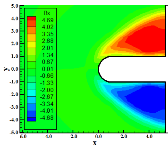
Figure 17. B_x component contours (Park-TV).
