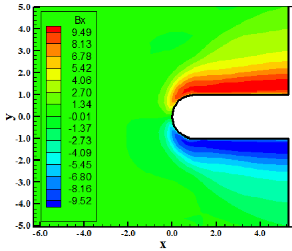
Figure 49. B_x component contours (Park-TV).
