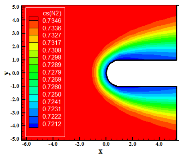
Figure 30. N_2 mass fraction contours (DK-TV).
