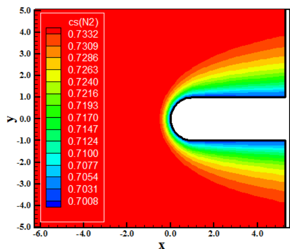
Figure 47. N_2 mass fraction contours (Park-TV).
