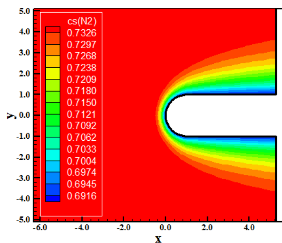
Figure 46. N_2 mass fraction contours (DK-TV).
