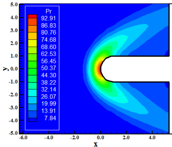
Figure 21. Pressure contours (Park-MAV).
