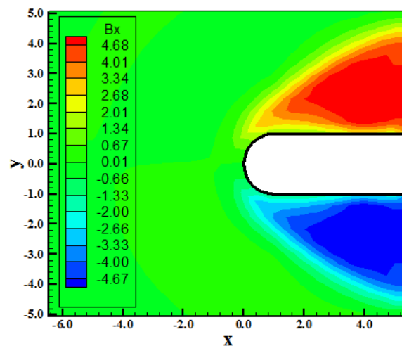
Figure 16. B_x component contours (DK-TV).
