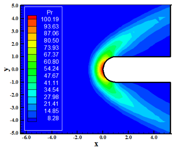
Figure 12. Pressure contours (DK-TV).
