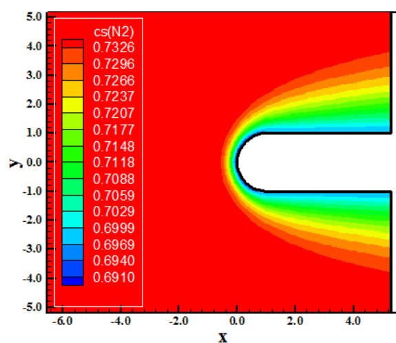
Figure 38. N_2 mass fraction contours (DK-MAV).
