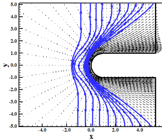
Figure 50. Induction lines (DK-TV).
