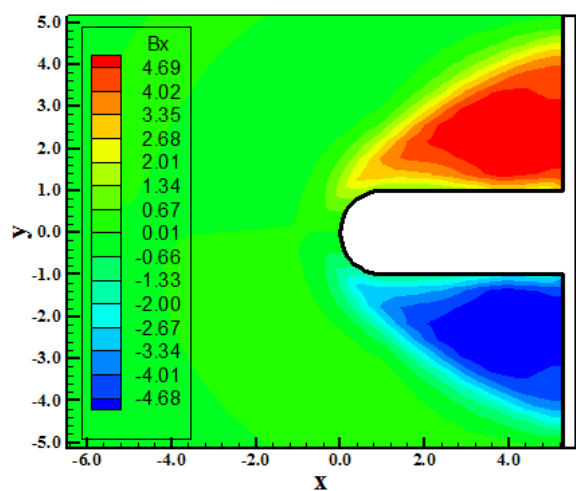
Figure 33. B x component contours (Park-TV).
