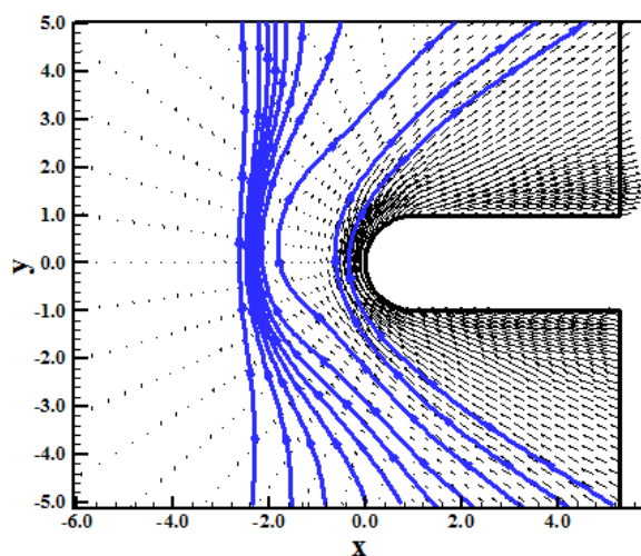
Figure 42. Induction lines (DK-MAV).
