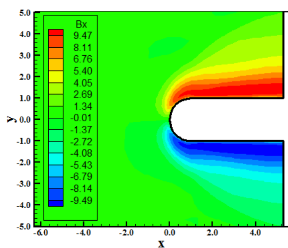
Figure 48. B_x component contours (DK-TV).
