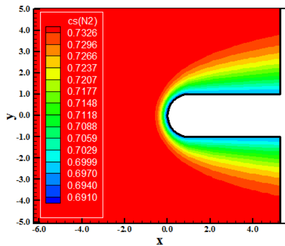
Figure 54. N_2 mass fraction contours (DK-MAV).
