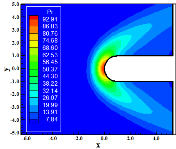
Figure 5. Pressure contours (Park-MAV).
