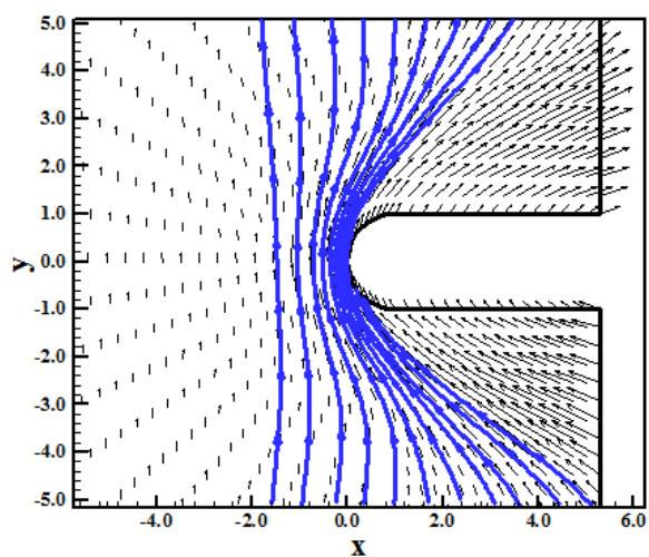
Figure 27. Induction lines (Park-MAV).
