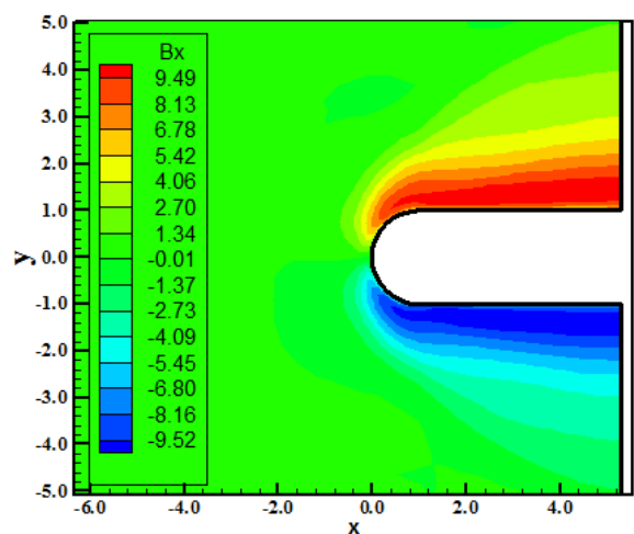
Figure 65. B_x component contours (Park-TV).
