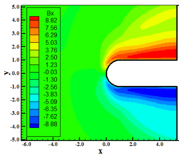
Figure 57. B_x component contours (Park-MAV).
