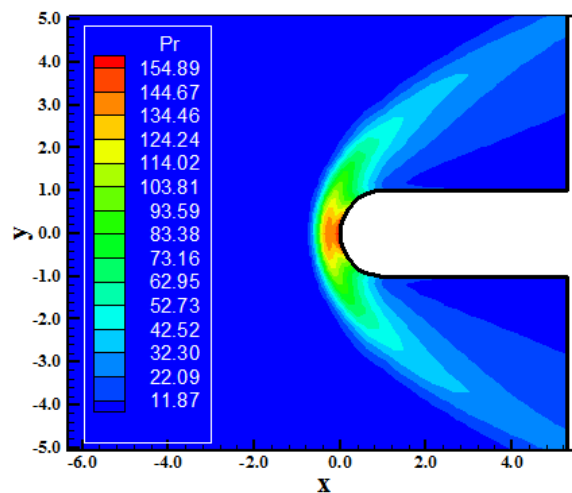
Figure 60. Pressure contours (DK-TV).
