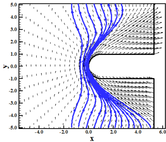
Figure 19. Induction lines (Park-TV).
