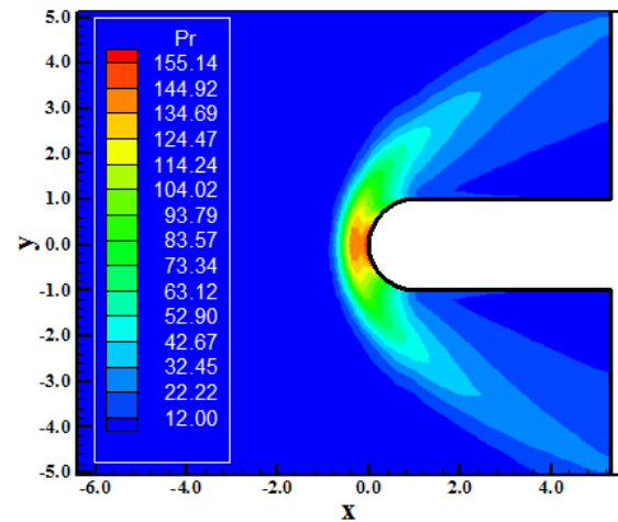
Figure 53. Pressure contours (Park-MAV).
