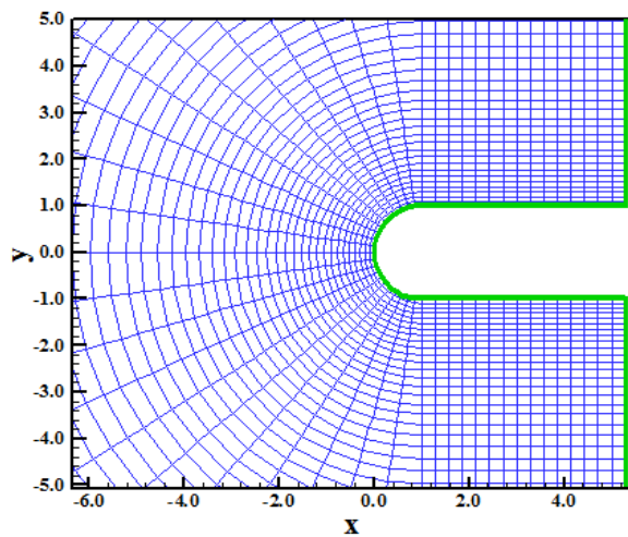
Figure 3. Blunt body viscous mesh.
