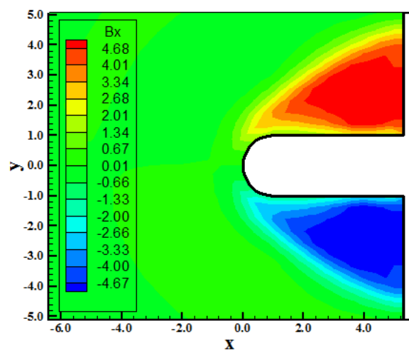
Figure 32. B x component contours (DK-TV).
