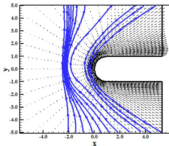
Figure 43. Induction lines (Park-MAV).
