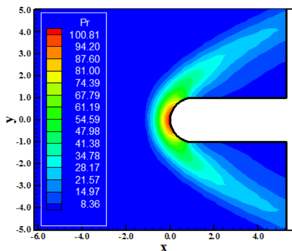
Figure 13. Pressure contours (Park-TV).
