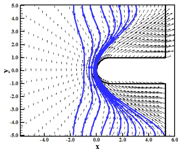
Figure 18. Induction lines (DK-TV).
