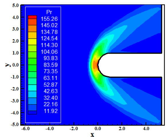
Figure 36. Pressure contours (DK-MAV).
