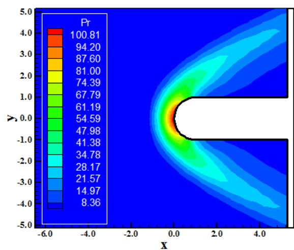
Figure 29. Pressure contours (Park-TV).
