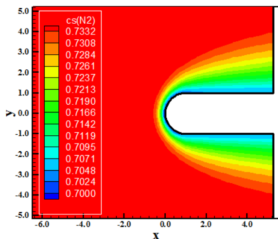
Figure 55. N_2 mass fraction contours (Park-MAV).
