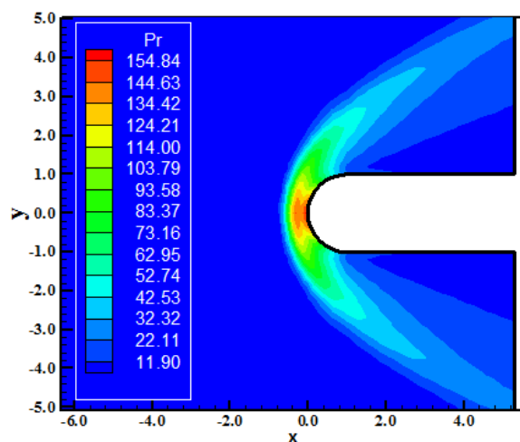
Figure 61. Pressure contours (Park-TV).
