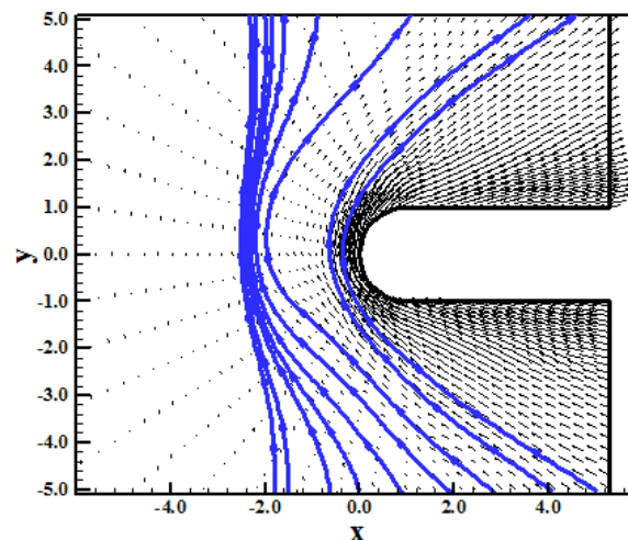
Figure 58. Induction lines (DK-MAV).
