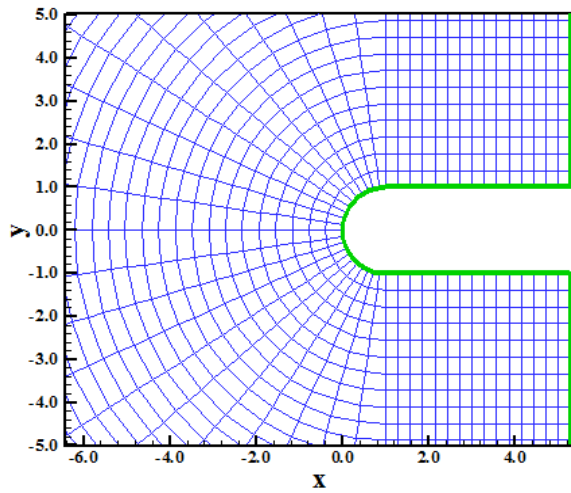
Figure 2. Blunt body inviscid mesh.
