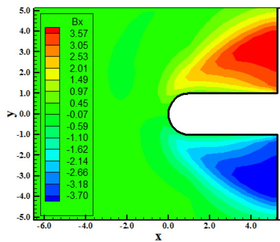
Figure 8. B x component contours (DK-MAV).
