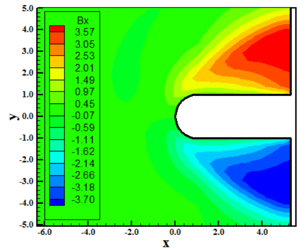
Figure 24. B_x component contours (DK-MAV).
