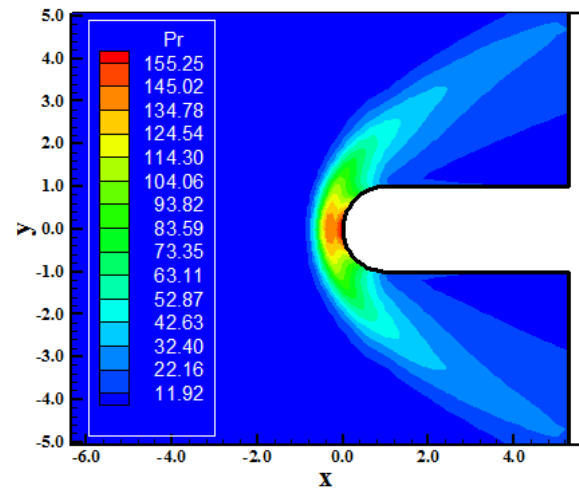
Figure 52. Pressure contours (DK-MAV)
