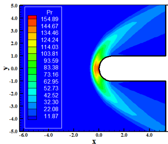
Figure 44. Pressure contours (DK-TV).
