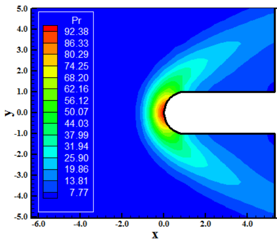
Figure 20. Pressure contours (DK-MAV).
