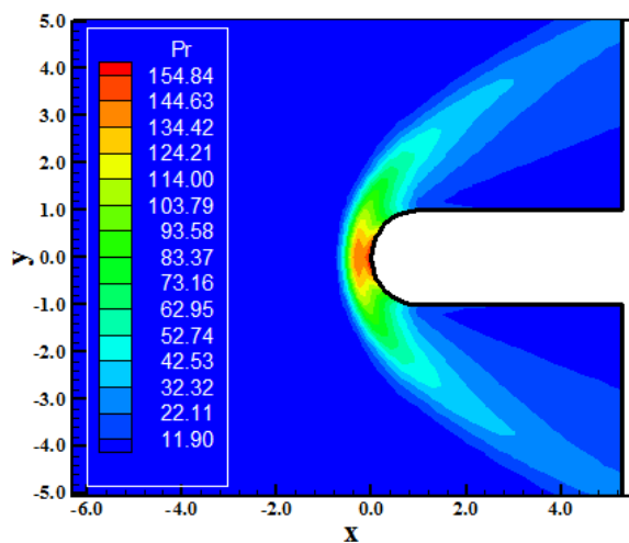
Figure 45. Pressure contours (Park-TV).
