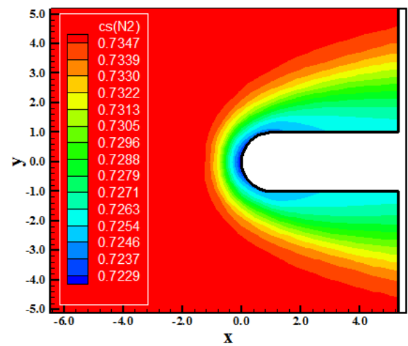
Figure 22. N_2 mass fraction contours (DK-MAV).
