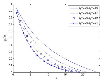
(b) The ruin probability of \psi_2(u) .
