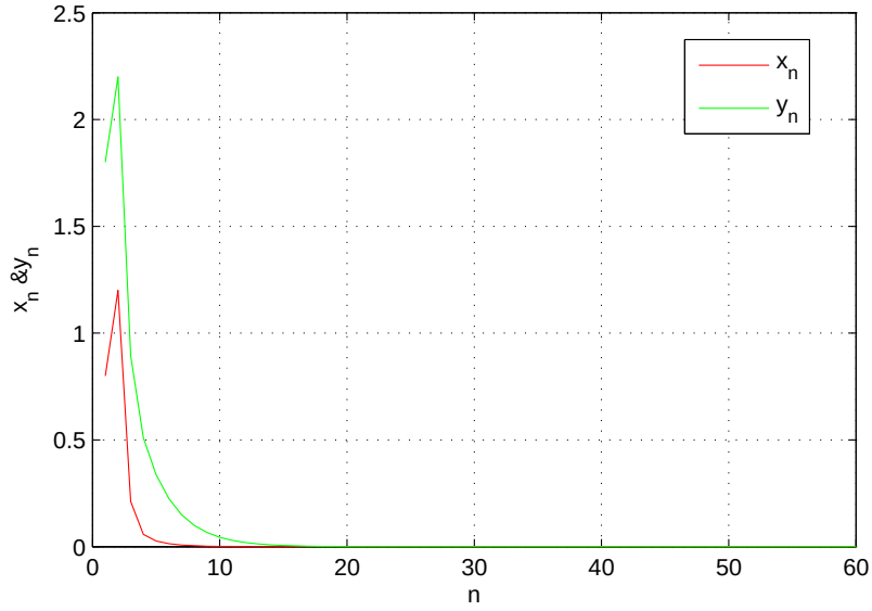
Fig.1. The plot of system (4.1).
