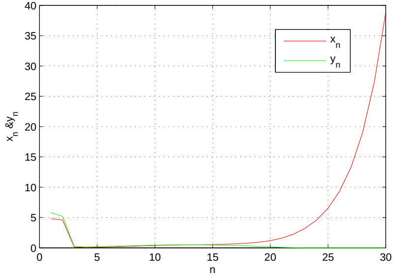
Fig.2. The plot of system (4.2).
