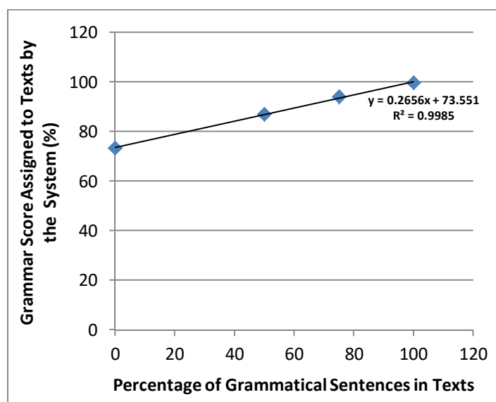
Figure 8: Regression chart of system-assigned grammar scores (in %) against percentage grammatical sentences in texts
