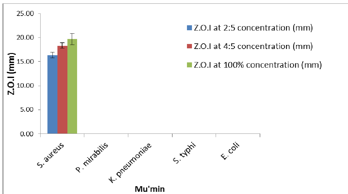
106 107 Figure 2. Zone of inhibition of Mu'min brand toothpaste against microorganisms.
