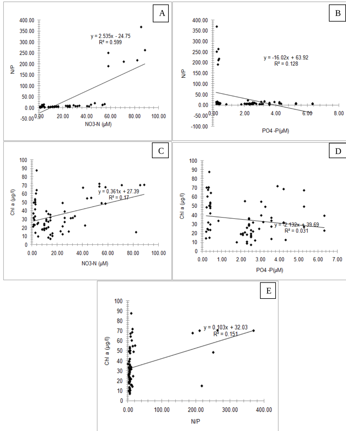
Figure 4: Relationships: A) N/P to NO 3 -N (μM); B) N/P to PO 4 -P (μM); C) Chl a (μg/l) to NO 3 -N; D) Chl a (μg/L) to PO 4 -P; E) Chl a (μg/L) to N/P; according to data collected in sample stations: GB, ChP, HB, EFQ, WChDC and CB.
